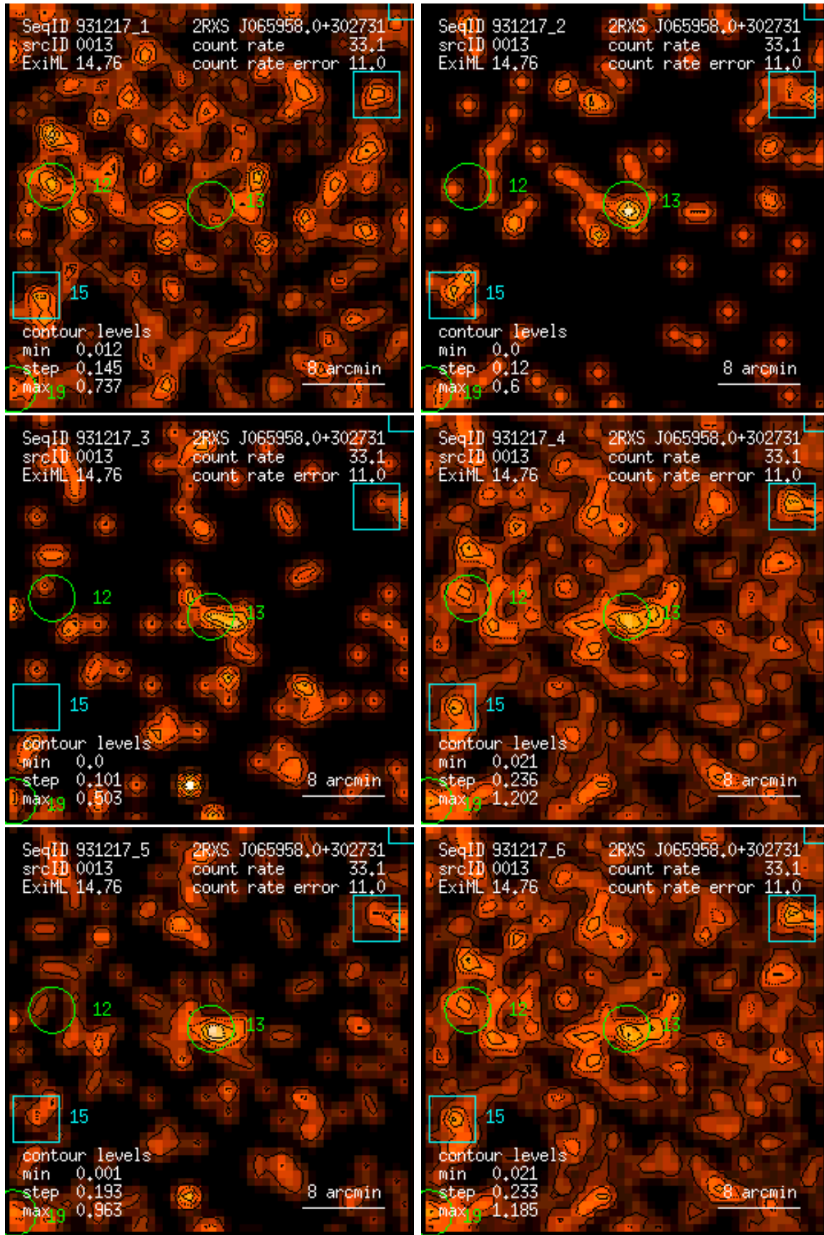
Figure 13: RASS 931217: detection 0013: band rate images, Gaussian filter: (1) PSPC channels 11 – 41, (2) 52 – 90, (3) 91 – 201, (4) 11 – 235, (5) 52 – 201, (6) 11 – 201. Broad band rates in counts/ks. Band rate contour levels in counts/ks/arcmin 2 .
