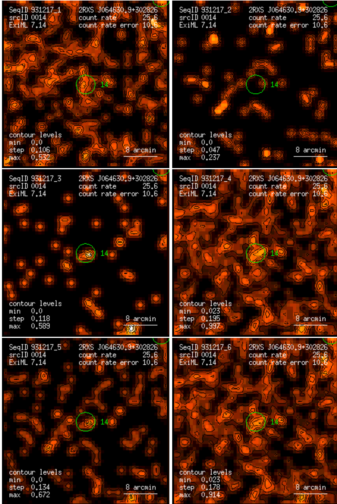
Figure 14: RASS 931217: detection 0014: band rate images, Gaussian filter: (1) PSPC channels 11 – 41, (2) 52 – 90, (3) 91 – 201, (4) 11 – 235, (5) 52 – 201, (6) 11 – 201. Broad band rates in counts/ks. Band rate contour levels in counts/ks/arcmin 2 .
