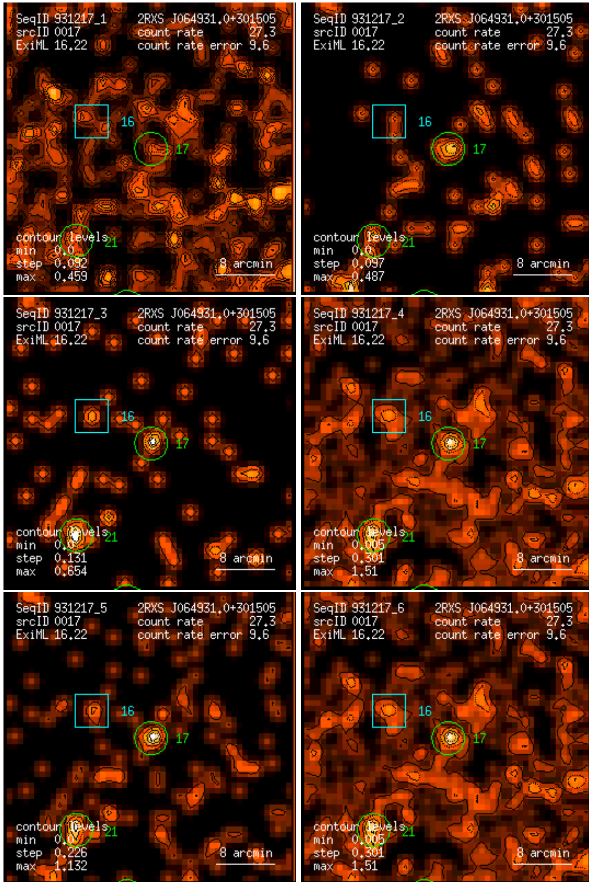
Figure 17: RASS 931217: detection 0017: band rate images, Gaussian filter: (1) PSPC channels 11 – 41, (2) 52 – 90, (3) 91 – 201, (4) 11 – 235, (5) 52 – 201, (6) 11 – 201. Broad band rates in counts/ks. Band rate contour levels in counts/ks/arcmin 2 .
