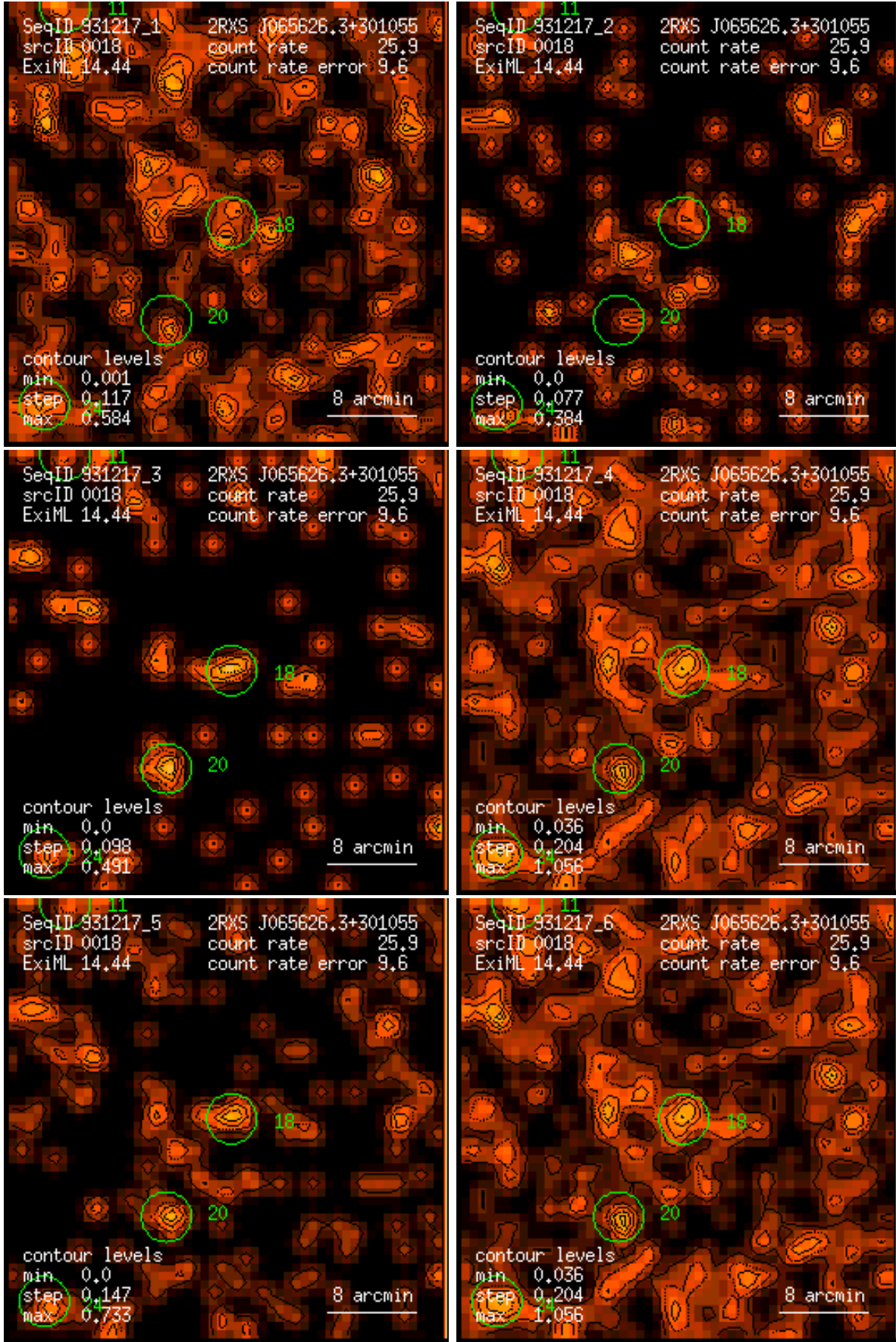
Figure 18: RASS 931217: detection 0018: band rate images, Gaussian filter: (1) PSPC channels 11 – 41, (2) 52 – 90, (3) 91 – 201, (4) 11 – 235, (5) 52 – 201, (6) 11 – 201. Broad band rates in counts/ks. Band rate contour levels in counts/ks/arcmin 2 .
