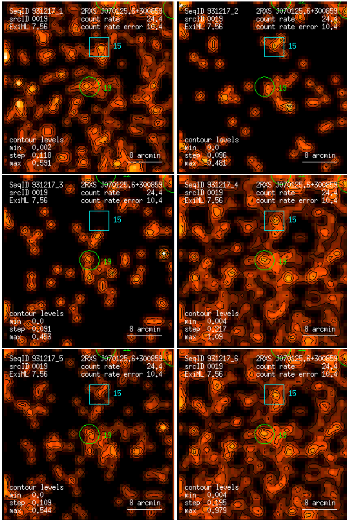
Figure 19: RASS 931217: detection 0019: band rate images, Gaussian filter: (1) PSPC channels 11 – 41, (2) 52 – 90, (3) 91 – 201, (4) 11 – 235, (5) 52 – 201, (6) 11 – 201. Broad band rates in counts/ks. Band rate contour levels in counts/ks/arcmin 2 .
