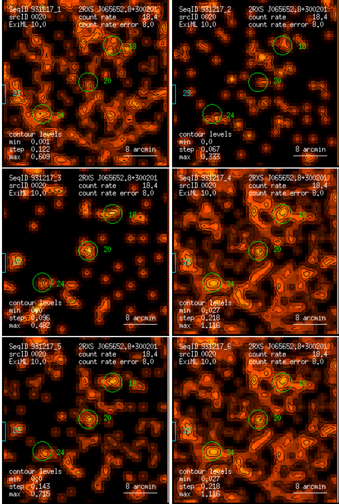
Figure 20: RASS 931217: detection 0020: band rate images, Gaussian filter: (1) PSPC channels 11 – 41, (2) 52 – 90, (3) 91 – 201, (4) 11 – 235, (5) 52 – 201, (6) 11 – 201. Broad band rates in counts/ks. Band rate contour levels in counts/ks/arcmin 2 .
