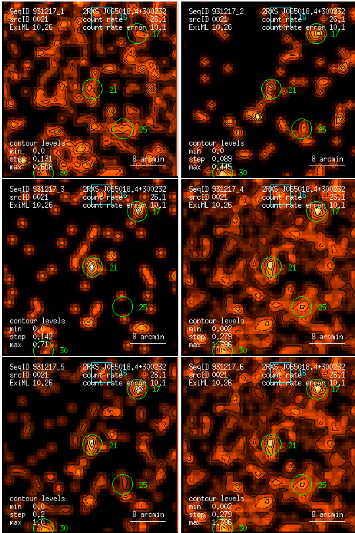
Figure 21: RASS 931217: detection 0021: band rate images, Gaussian filter: (1) PSPC channels 11 – 41, (2) 52 – 90, (3) 91 – 201, (4) 11 – 235, (5) 52 – 201, (6) 11 – 201. Broad band rates in counts/ks. Band rate contour levels in counts/ks/arcmin 2 .
