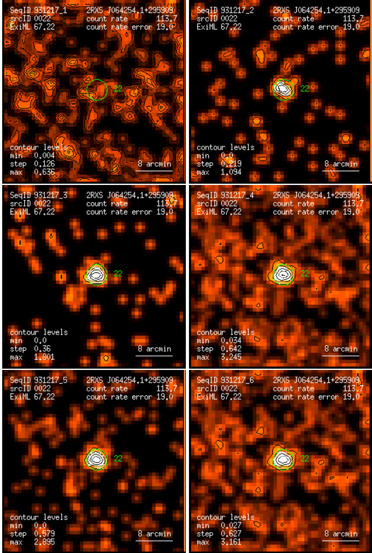
Figure 22: RASS 931217: detection 0022: band rate images, Gaussian filter: (1) PSPC channels 11 – 41, (2) 52 – 90, (3) 91 – 201, (4) 11 – 235, (5) 52 – 201, (6) 11 – 201. Broad band rates in counts/ks. Band rate contour levels in counts/ks/arcmin 2 .
