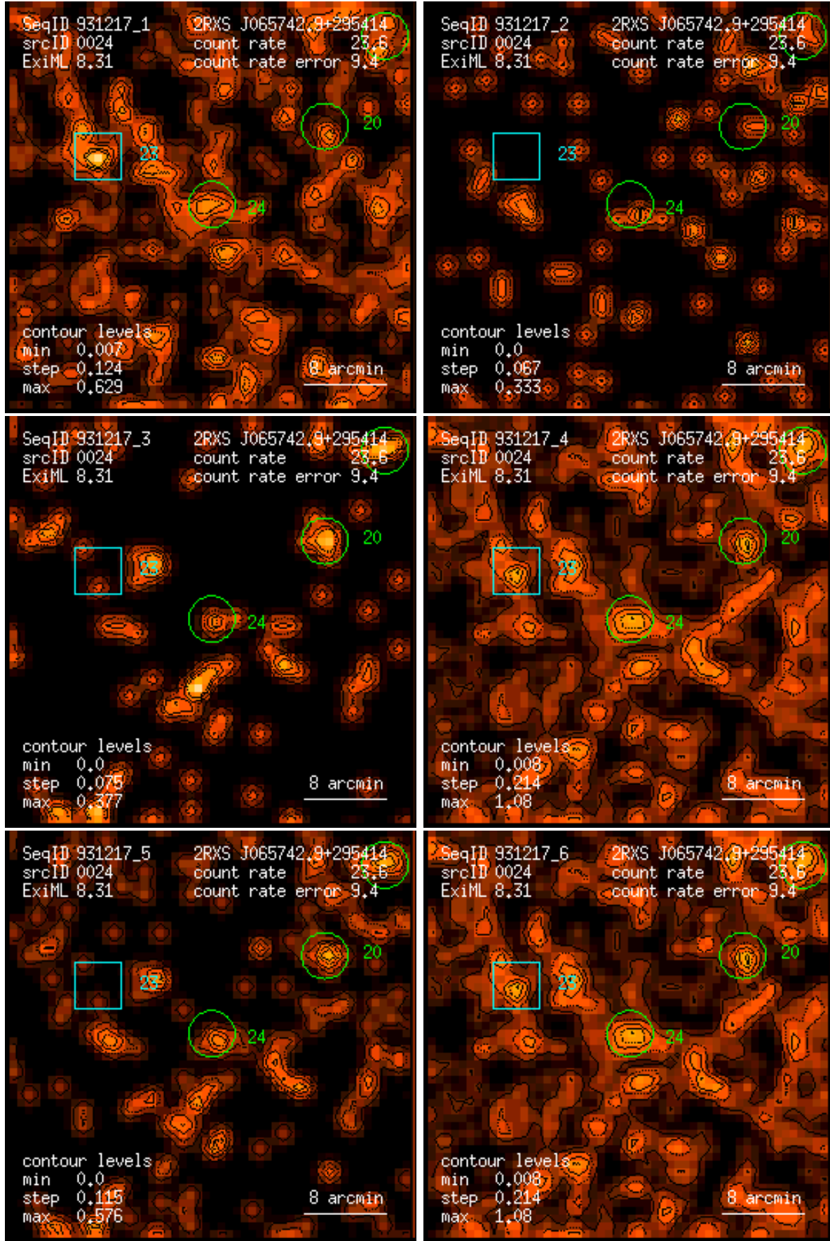
Figure 24: RASS 931217: detection 0024: band rate images, Gaussian filter: (1) PSPC channels 11 – 41, (2) 52 – 90, (3) 91 – 201, (4) 11 – 235, (5) 52 – 201, (6) 11 – 201. Broad band rates in counts/ks. Band rate contour levels in counts/ks/arcmin 2 .
