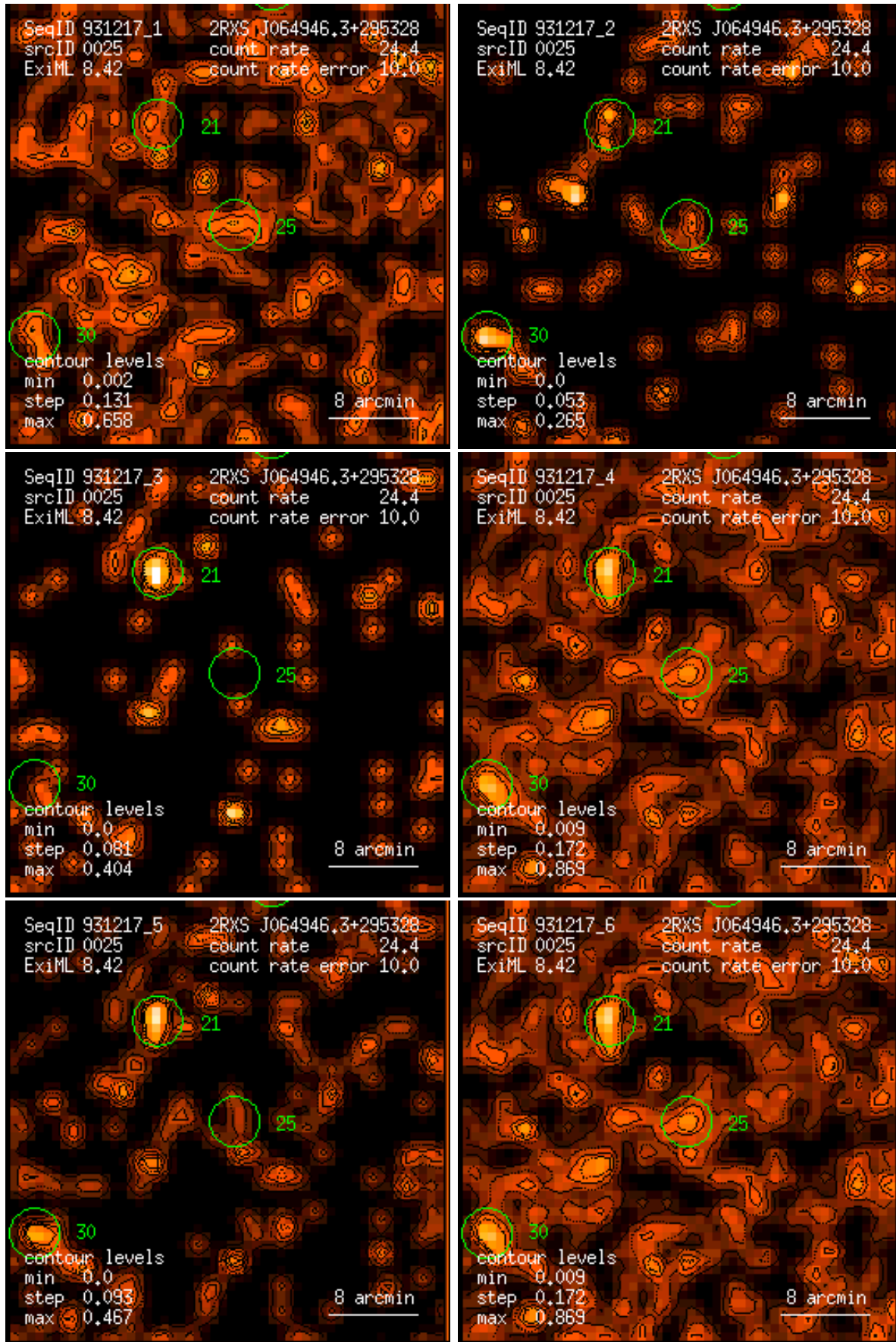
Figure 25: RASS 931217: detection 0025: band rate images, Gaussian filter: (1) PSPC channels 11 – 41, (2) 52 – 90, (3) 91 – 201, (4) 11 – 235, (5) 52 – 201, (6) 11 – 201. Broad band rates in counts/ks. Band rate contour levels in counts/ks/arcmin 2 .
