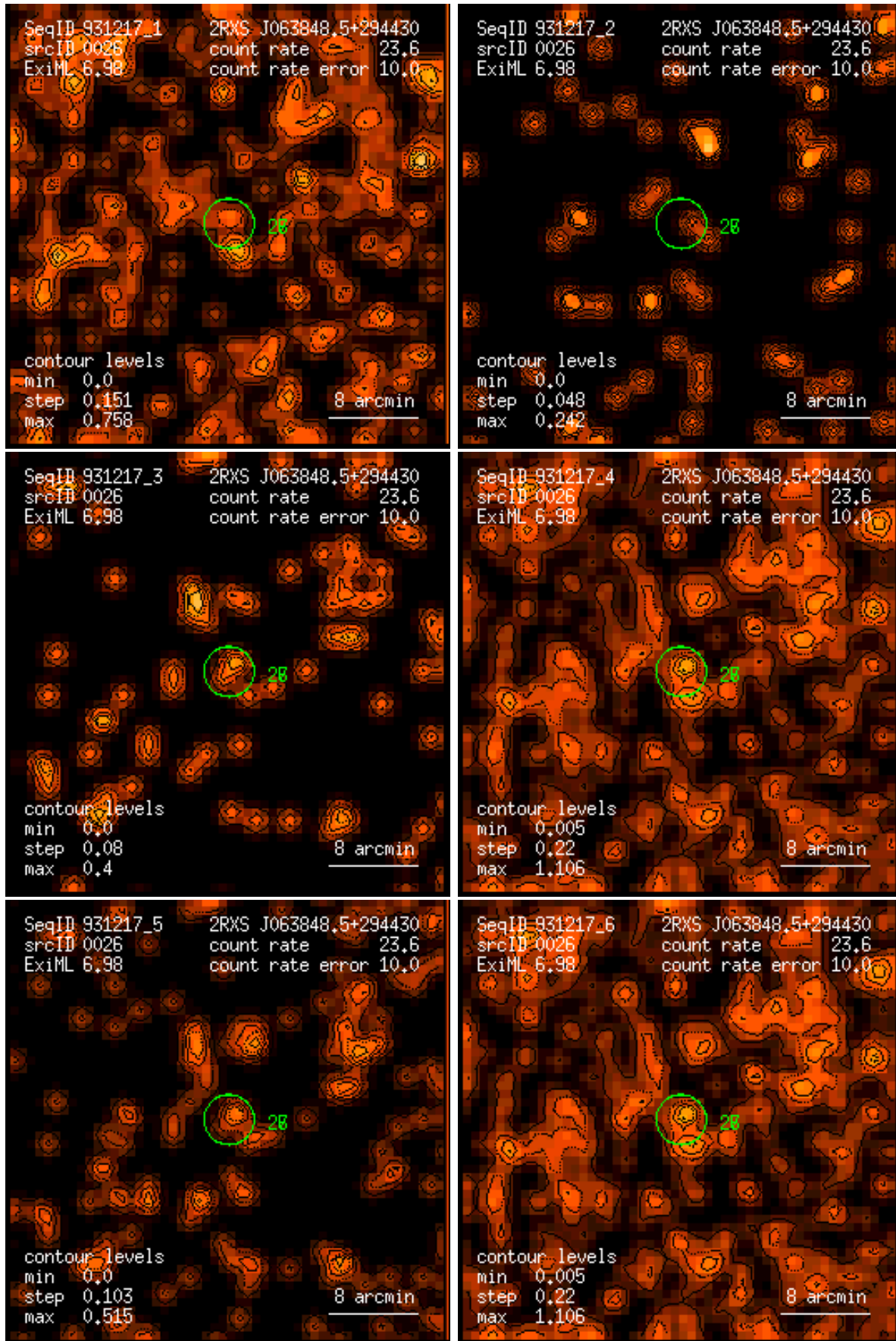
Figure 26: RASS 931217: detection 0026: band rate images, Gaussian filter: (1) PSPC channels 11 – 41, (2) 52 – 90, (3) 91 – 201, (4) 11 – 235, (5) 52 – 201, (6) 11 – 201. Broad band rates in counts/ks. Band rate contour levels in counts/ks/arcmin 2 .
