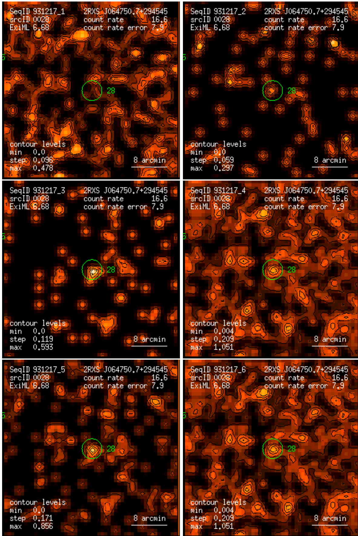
Figure 28: RASS 931217: detection 0028: band rate images, Gaussian filter: (1) PSPC channels 11 – 41, (2) 52 – 90, (3) 91 – 201, (4) 11 – 235, (5) 52 – 201, (6) 11 – 201. Broad band rates in counts/ks. Band rate contour levels in counts/ks/arcmin 2 .
