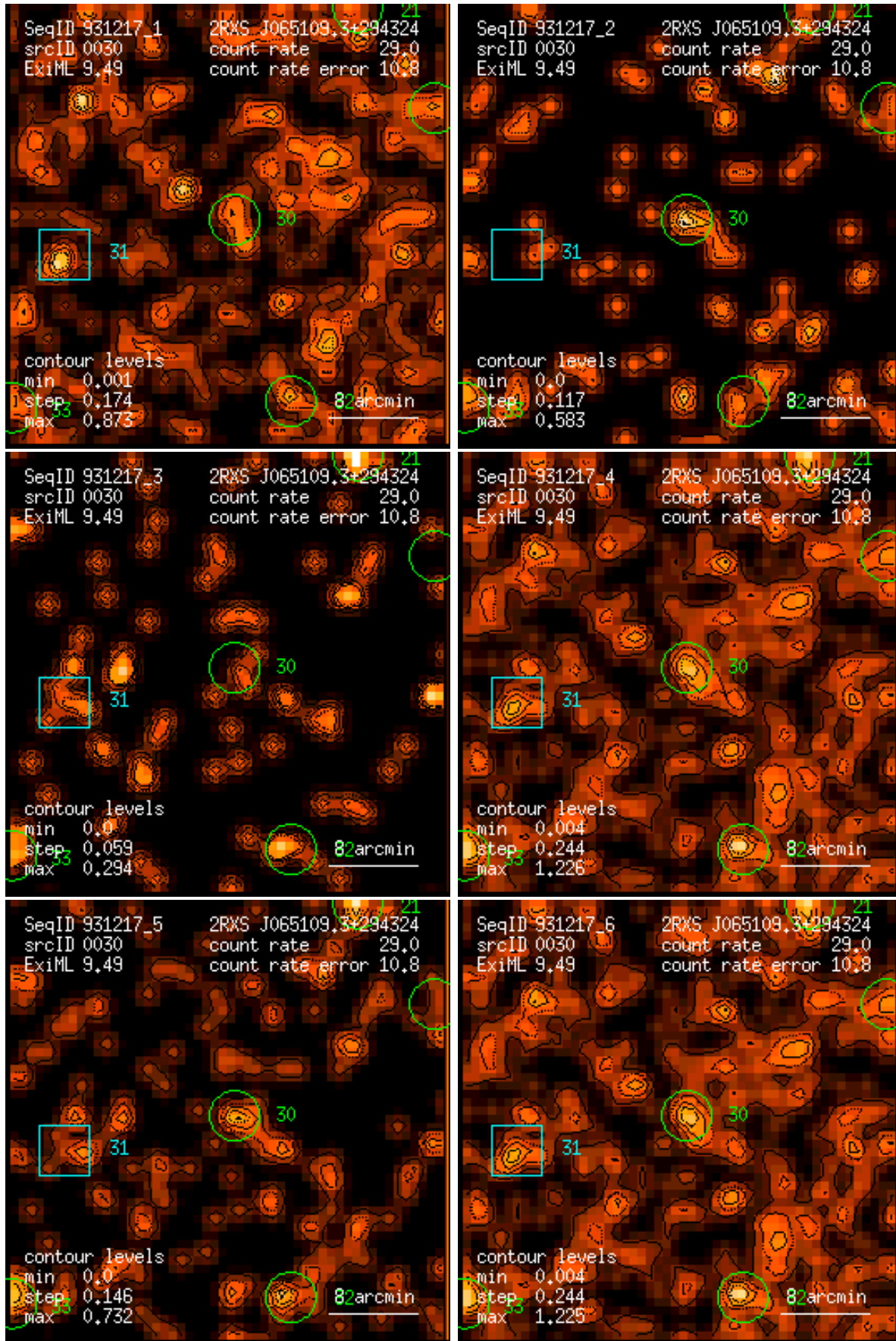
Figure 30: RASS 931217: detection 0030: band rate images, Gaussian filter: (1) PSPC channels 11 – 41, (2) 52 – 90, (3) 91 – 201, (4) 11 – 235, (5) 52 – 201, (6) 11 – 201. Broad band rates in counts/ks. Band rate contour levels in counts/ks/arcmin 2 .
