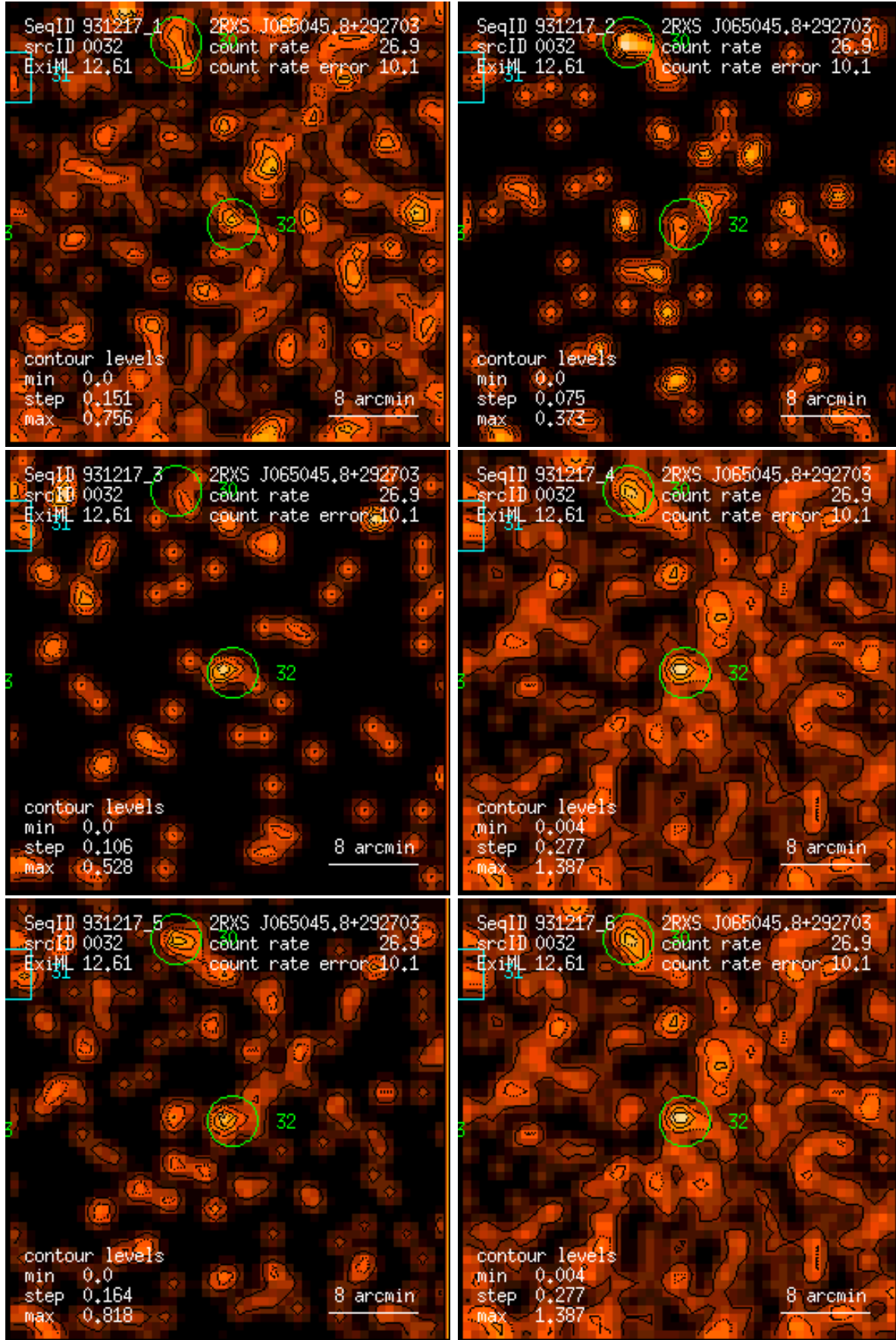
Figure 32: RASS 931217: detection 0032: band rate images, Gaussian filter: (1) PSPC channels 11 – 41, (2) 52 – 90, (3) 91 – 201, (4) 11 – 235, (5) 52 – 201, (6) 11 – 201. Broad band rates in counts/ks. Band rate contour levels in counts/ks/arcmin 2 .
