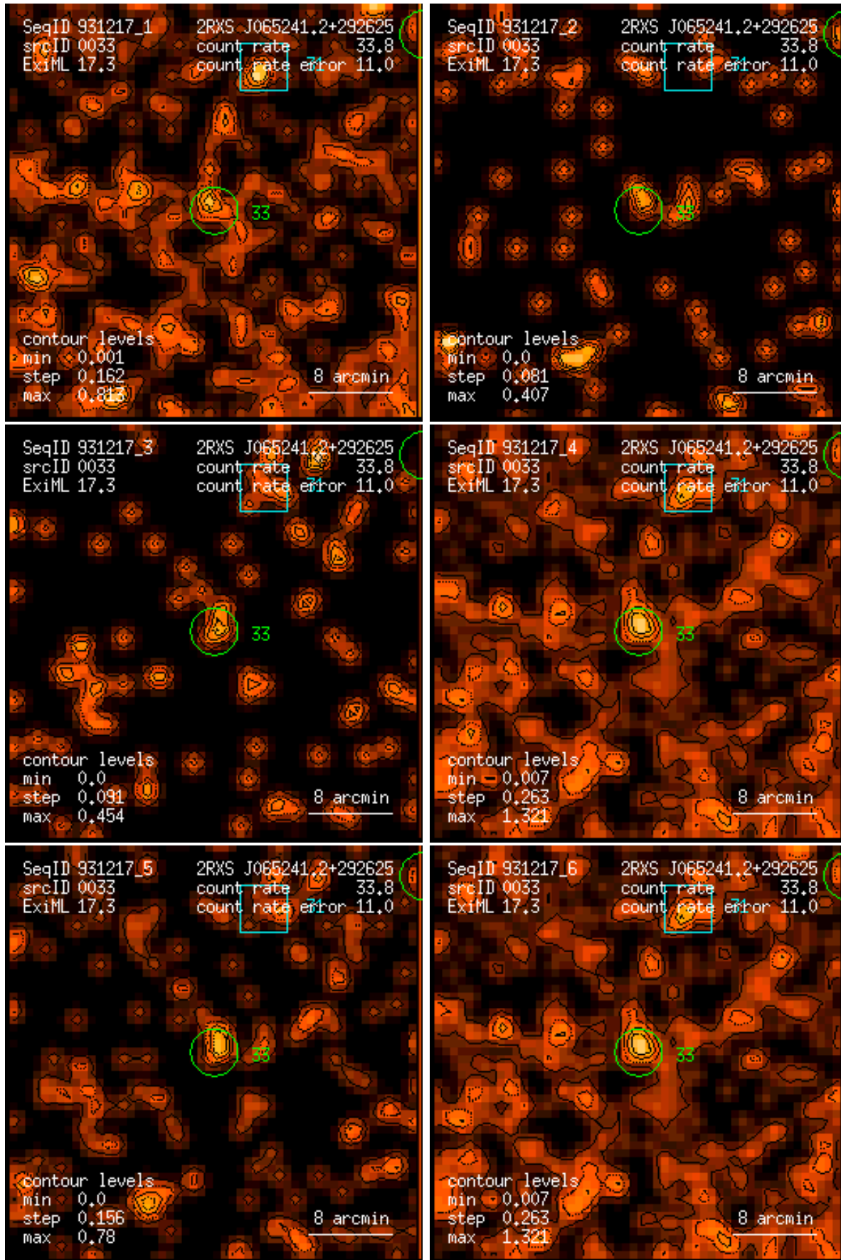
Figure 33: RASS 931217: detection 0033: band rate images, Gaussian filter: (1) PSPC channels 11 – 41, (2) 52 – 90, (3) 91 – 201, (4) 11 – 235, (5) 52 – 201, (6) 11 – 201. Broad band rates in counts/ks. Band rate contour levels in counts/ks/arcmin 2 .
