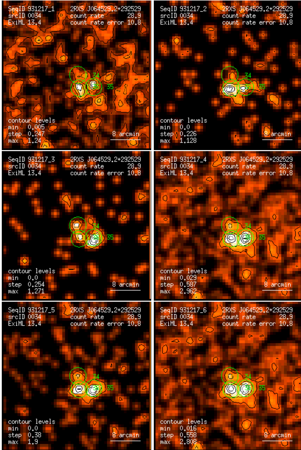
Figure 34: RASS 931217: detection 0034: band rate images, Gaussian filter: (1) PSPC channels 11 – 41, (2) 52 – 90, (3) 91 – 201, (4) 11 – 235, (5) 52 – 201, (6) 11 – 201. Broad band rates in counts/ks. Band rate contour levels in counts/ks/arcmin 2 .
