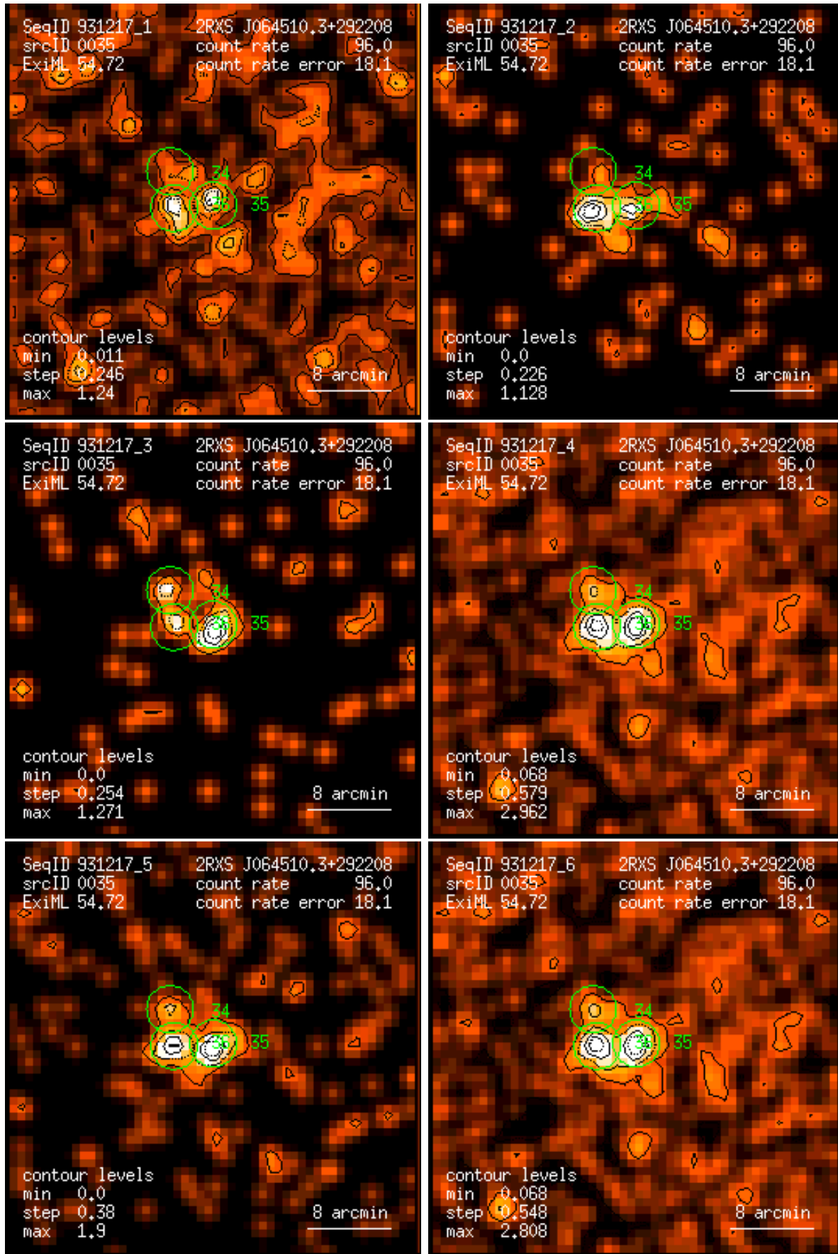
Figure 35: RASS 931217: detection 0035: band rate images, Gaussian filter: (1) PSPC channels 11 – 41, (2) 52 – 90, (3) 91 – 201, (4) 11 – 235, (5) 52 – 201, (6) 11 – 201. Broad band rates in counts/ks. Band rate contour levels in counts/ks/arcmin 2 .
