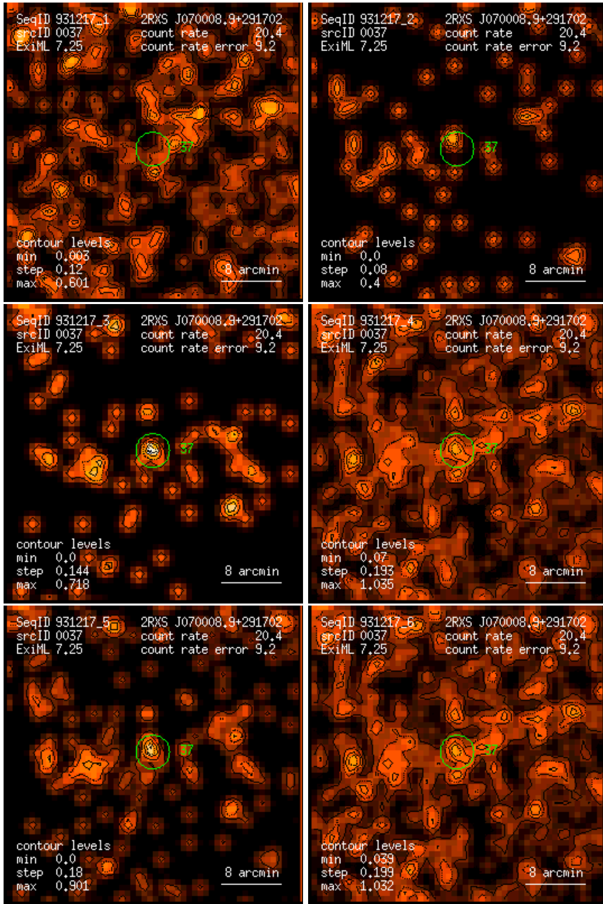
Figure 37: RASS 931217: detection 0037: band rate images, Gaussian filter: (1) PSPC channels 11 – 41, (2) 52 – 90, (3) 91 – 201, (4) 11 – 235, (5) 52 – 201, (6) 11 – 201. Broad band rates in counts/ks. Band rate contour levels in counts/ks/arcmin 2 .
