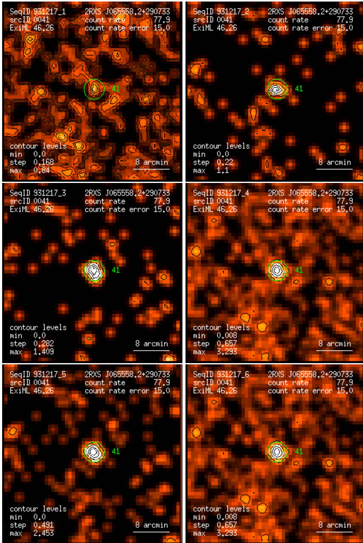
Figure 41: RASS 931217: detection 0041: band rate images, Gaussian filter: (1) PSPC channels 11 – 41, (2) 52 – 90, (3) 91 – 201, (4) 11 – 235, (5) 52 – 201, (6) 11 – 201. Broad band rates in counts/ks. Band rate contour levels in counts/ks/arcmin 2 .
