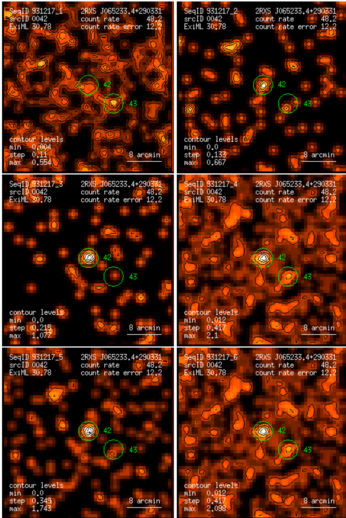
Figure 42: RASS 931217: detection 0042: band rate images, Gaussian filter: (1) PSPC channels 11 – 41, (2) 52 – 90, (3) 91 – 201, (4) 11 – 235, (5) 52 – 201, (6) 11 – 201. Broad band rates in counts/ks. Band rate contour levels in counts/ks/arcmin 2 .
