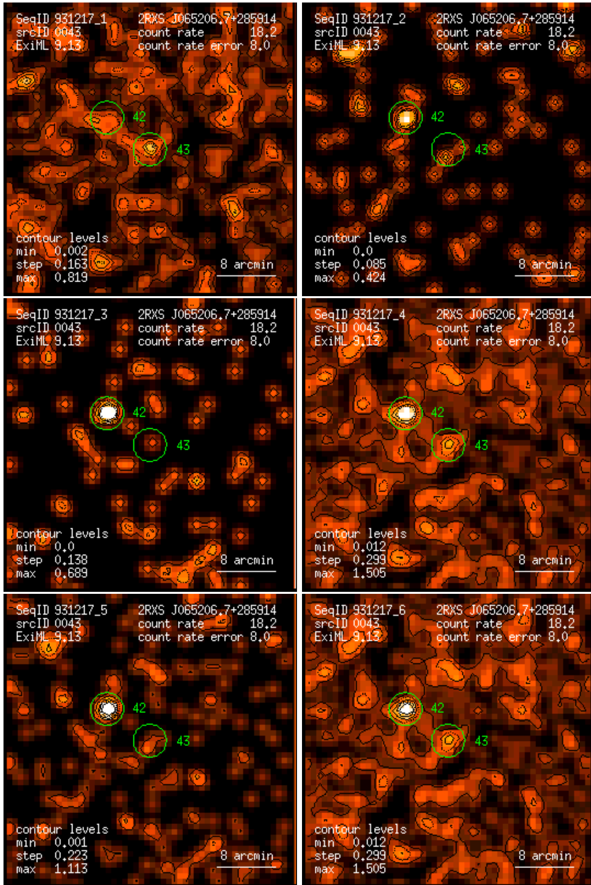
Figure 43: RASS 931217: detection 0043: band rate images, Gaussian filter: (1) PSPC channels 11 – 41, (2) 52 – 90, (3) 91 – 201, (4) 11 – 235, (5) 52 – 201, (6) 11 – 201. Broad band rates in counts/ks. Band rate contour levels in counts/ks/arcmin 2 .
