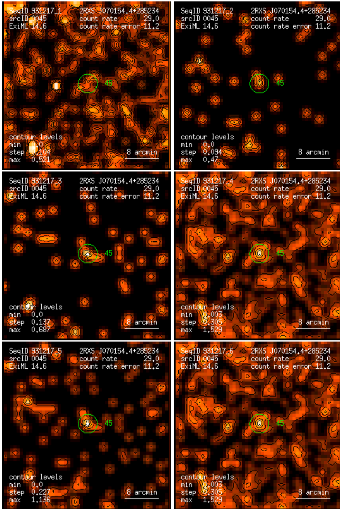
Figure 45: RASS 931217: detection 0045: band rate images, Gaussian filter: (1) PSPC channels 11 – 41, (2) 52 – 90, (3) 91 – 201, (4) 11 – 235, (5) 52 – 201, (6) 11 – 201. Broad band rates in counts/ks. Band rate contour levels in counts/ks/arcmin 2 .
