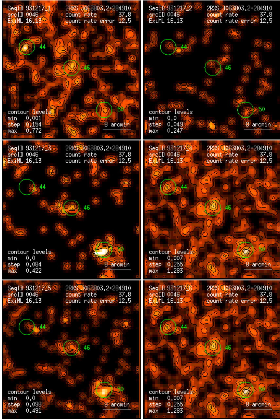
Figure 46: RASS 931217: detection 0046: band rate images, Gaussian filter: (1) PSPC channels 11 – 41, (2) 52 – 90, (3) 91 – 201, (4) 11 – 235, (5) 52 – 201, (6) 11 – 201. Broad band rates in counts/ks. Band rate contour levels in counts/ks/arcmin 2 .
