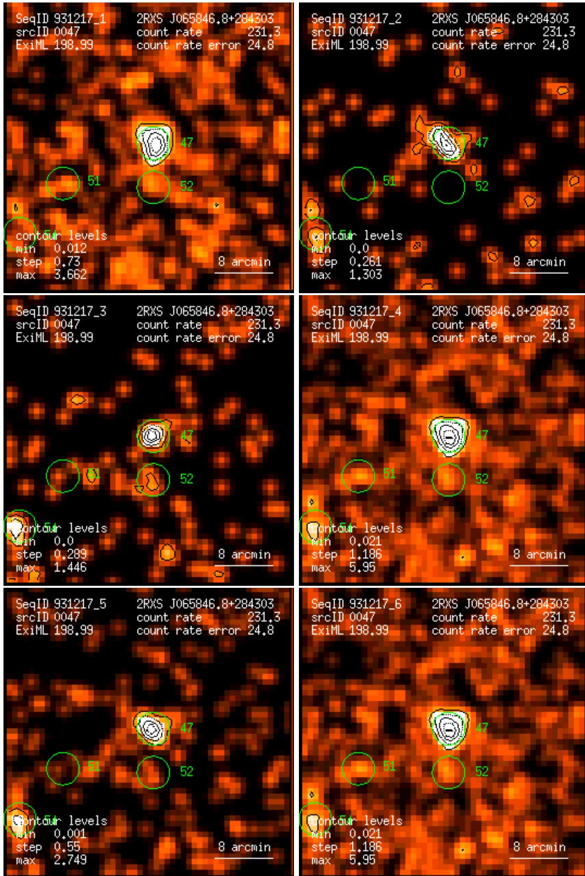
Figure 47: RASS 931217: detection 0047: band rate images, Gaussian filter: (1) PSPC channels 11 – 41, (2) 52 – 90, (3) 91 – 201, (4) 11 – 235, (5) 52 – 201, (6) 11 – 201. Broad band rates in counts/ks. Band rate contour levels in counts/ks/arcmin 2 .
