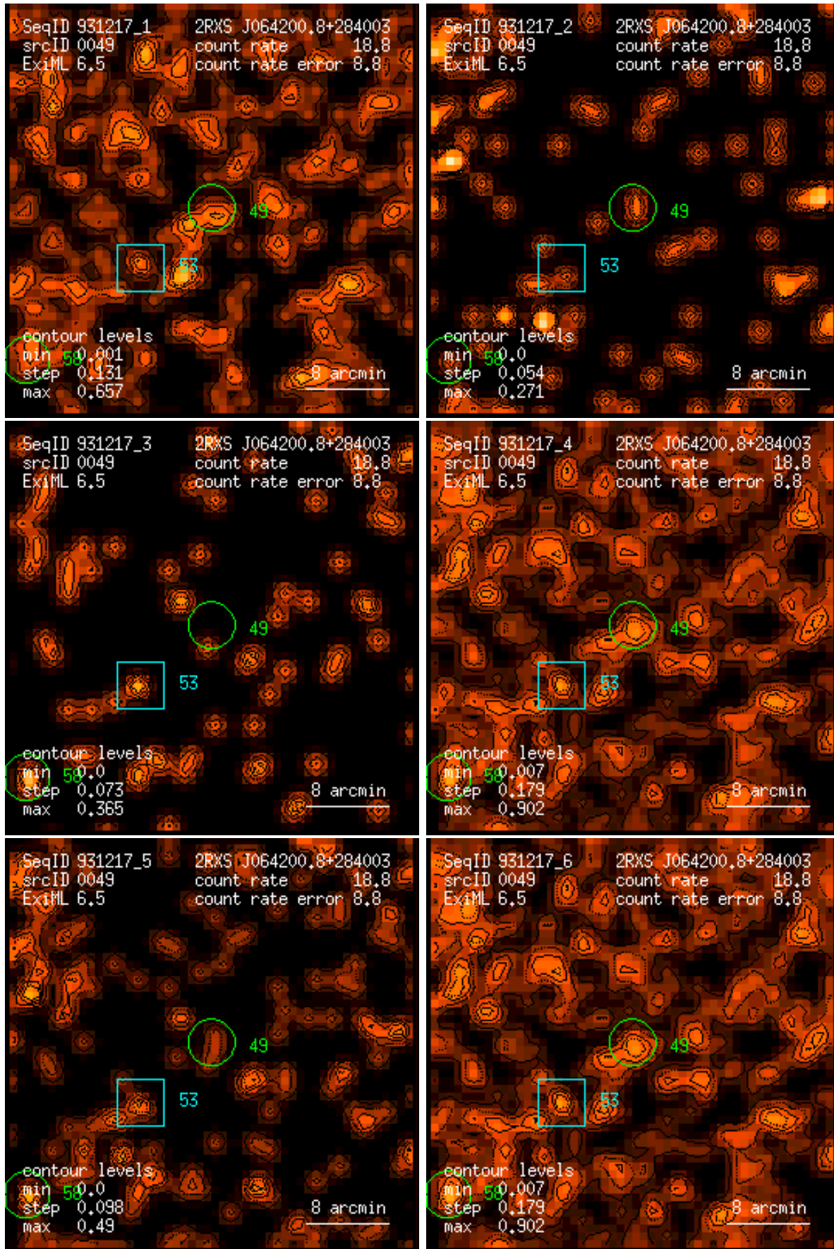
Figure 49: RASS 931217: detection 0049: band rate images, Gaussian filter: (1) PSPC channels 11 – 41, (2) 52 – 90, (3) 91 – 201, (4) 11 – 235, (5) 52 – 201, (6) 11 – 201. Broad band rates in counts/ks. Band rate contour levels in counts/ks/arcmin 2 .
