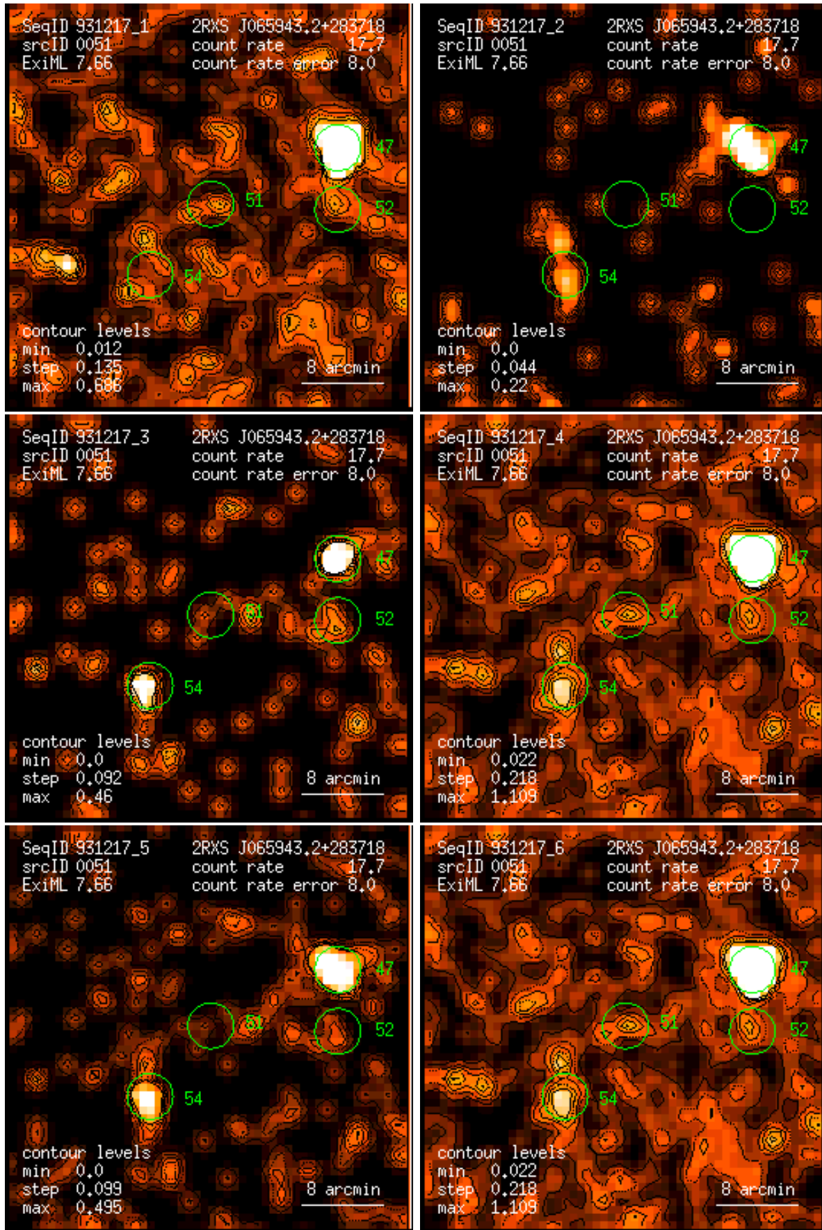
Figure 51: RASS 931217: detection 0051: band rate images, Gaussian filter: (1) PSPC channels 11 – 41, (2) 52 – 90, (3) 91 – 201, (4) 11 – 235, (5) 52 – 201, (6) 11 – 201. Broad band rates in counts/ks. Band rate contour levels in counts/ks/arcmin 2 .
