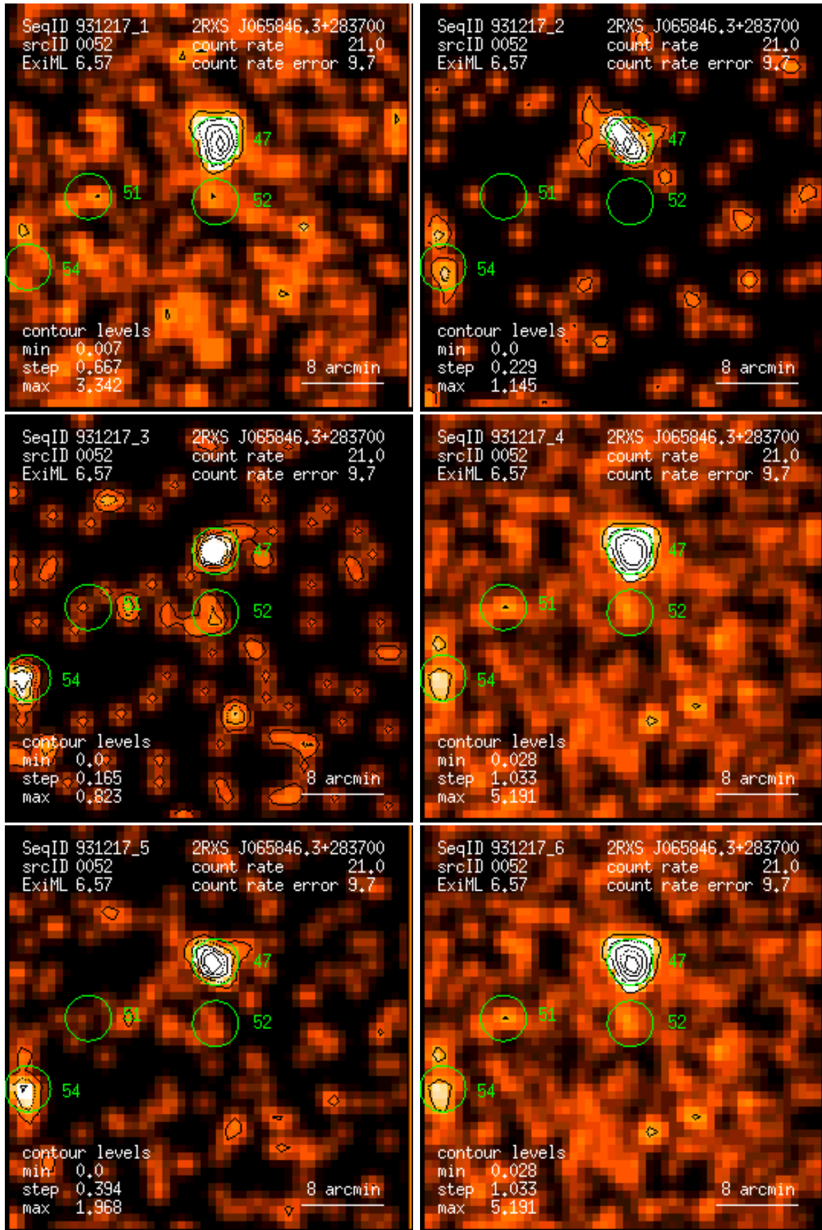
Figure 52: RASS 931217: detection 0052: band rate images, Gaussian filter: (1) PSPC channels 11 – 41, (2) 52 – 90, (3) 91 – 201, (4) 11 – 235, (5) 52 – 201, (6) 11 – 201. Broad band rates in counts/ks. Band rate contour levels in counts/ks/arcmin 2 .
