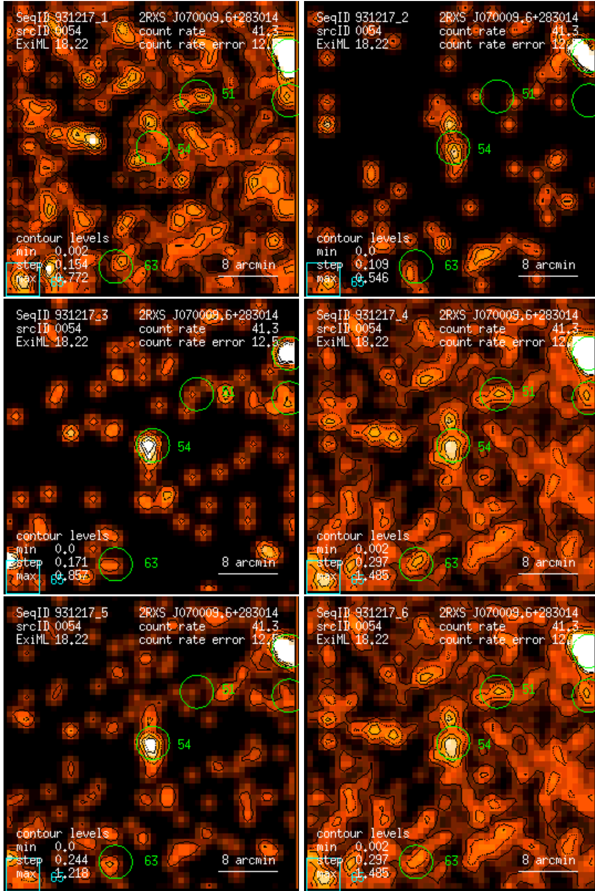
Figure 54: RASS 931217: detection 0054: band rate images, Gaussian filter: (1) PSPC channels 11 – 41, (2) 52 – 90, (3) 91 – 201, (4) 11 – 235, (5) 52 – 201, (6) 11 – 201. Broad band rates in counts/ks. Band rate contour levels in counts/ks/arcmin 2 .
