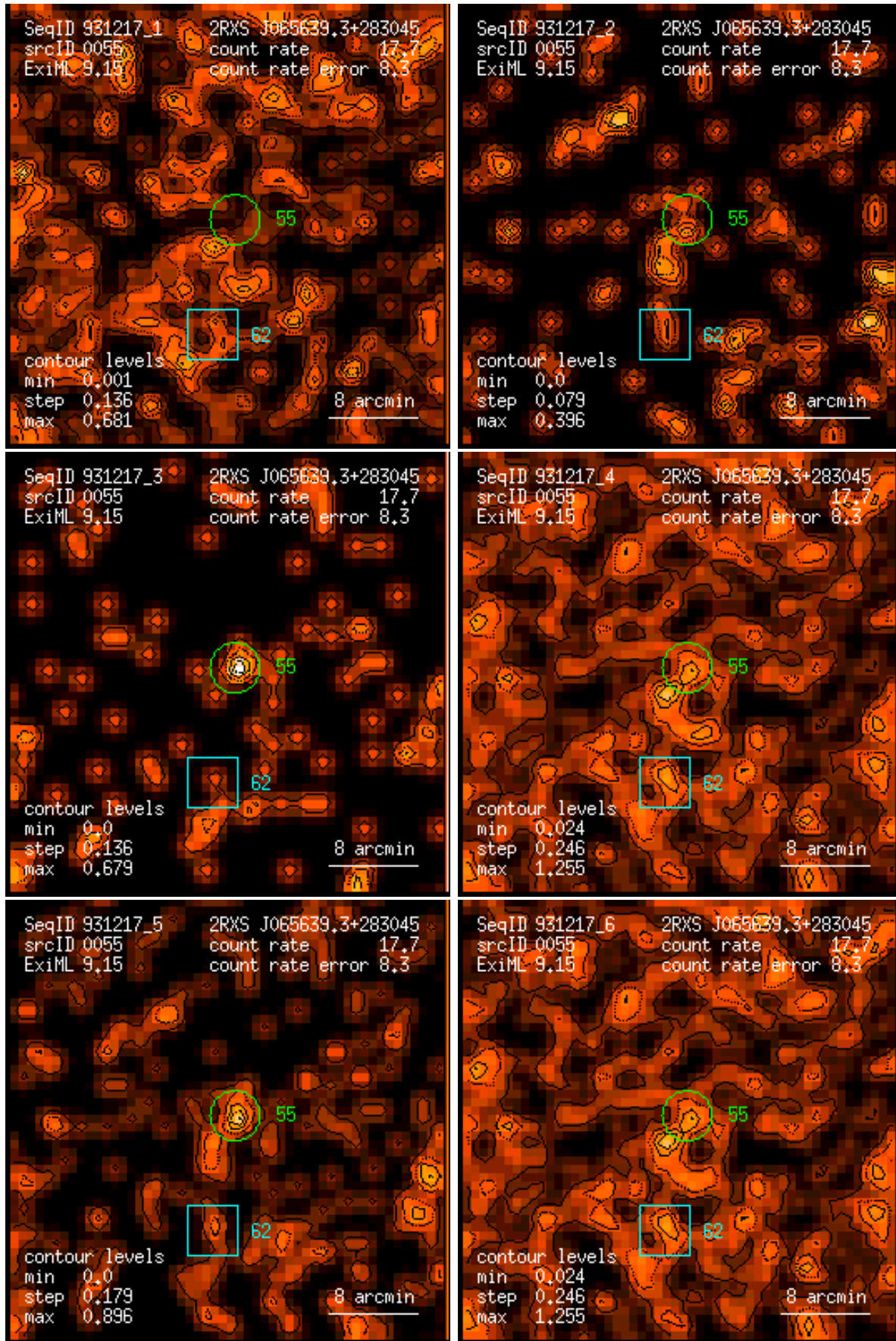
Figure 55: RASS 931217: detection 0055: band rate images, Gaussian filter: (1) PSPC channels 11 – 41, (2) 52 – 90, (3) 91 – 201, (4) 11 – 235, (5) 52 – 201, (6) 11 – 201. Broad band rates in counts/ks. Band rate contour levels in counts/ks/arcmin 2 .
