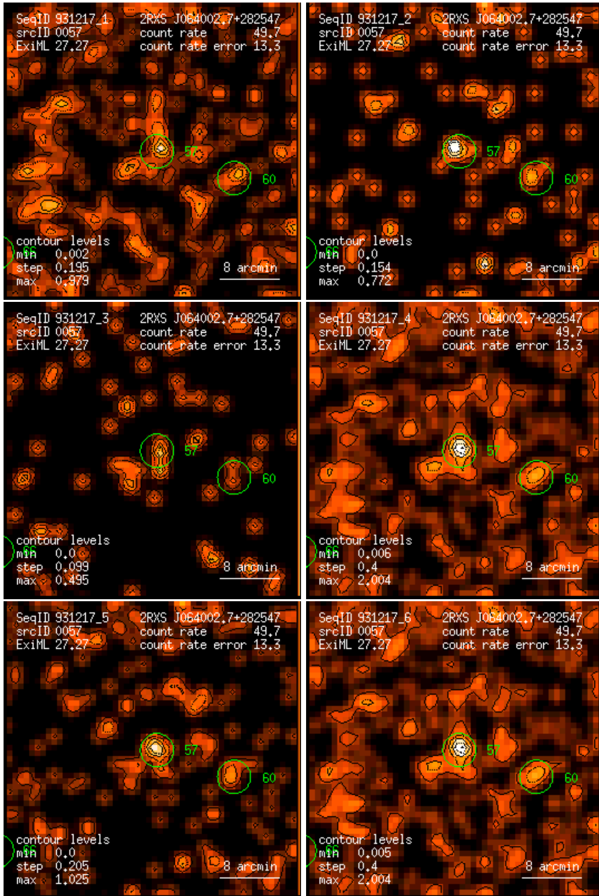
Figure 57: RASS 931217: detection 0057: band rate images, Gaussian filter: (1) PSPC channels 11 – 41, (2) 52 – 90, (3) 91 – 201, (4) 11 – 235, (5) 52 – 201, (6) 11 – 201. Broad band rates in counts/ks. Band rate contour levels in counts/ks/arcmin 2 .
