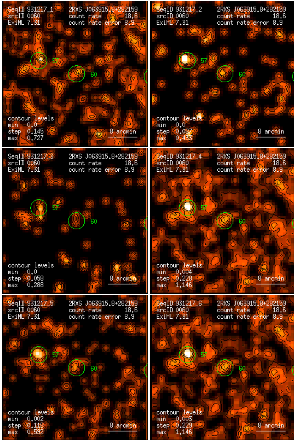
Figure 60: RASS 931217: detection 0060: band rate images, Gaussian filter: (1) PSPC channels 11 – 41, (2) 52 – 90, (3) 91 – 201, (4) 11 – 235, (5) 52 – 201, (6) 11 – 201. Broad band rates in counts/ks. Band rate contour levels in counts/ks/arcmin 2 .
