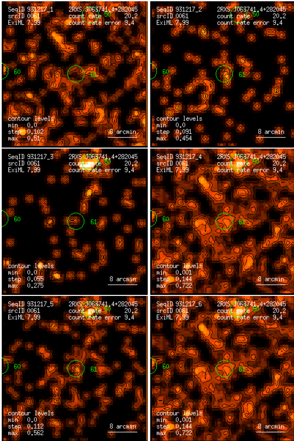
Figure 61: RASS 931217: detection 0061: band rate images, Gaussian filter: (1) PSPC channels 11 – 41, (2) 52 – 90, (3) 91 – 201, (4) 11 – 235, (5) 52 – 201, (6) 11 – 201. Broad band rates in counts/ks. Band rate contour levels in counts/ks/arcmin 2 .
