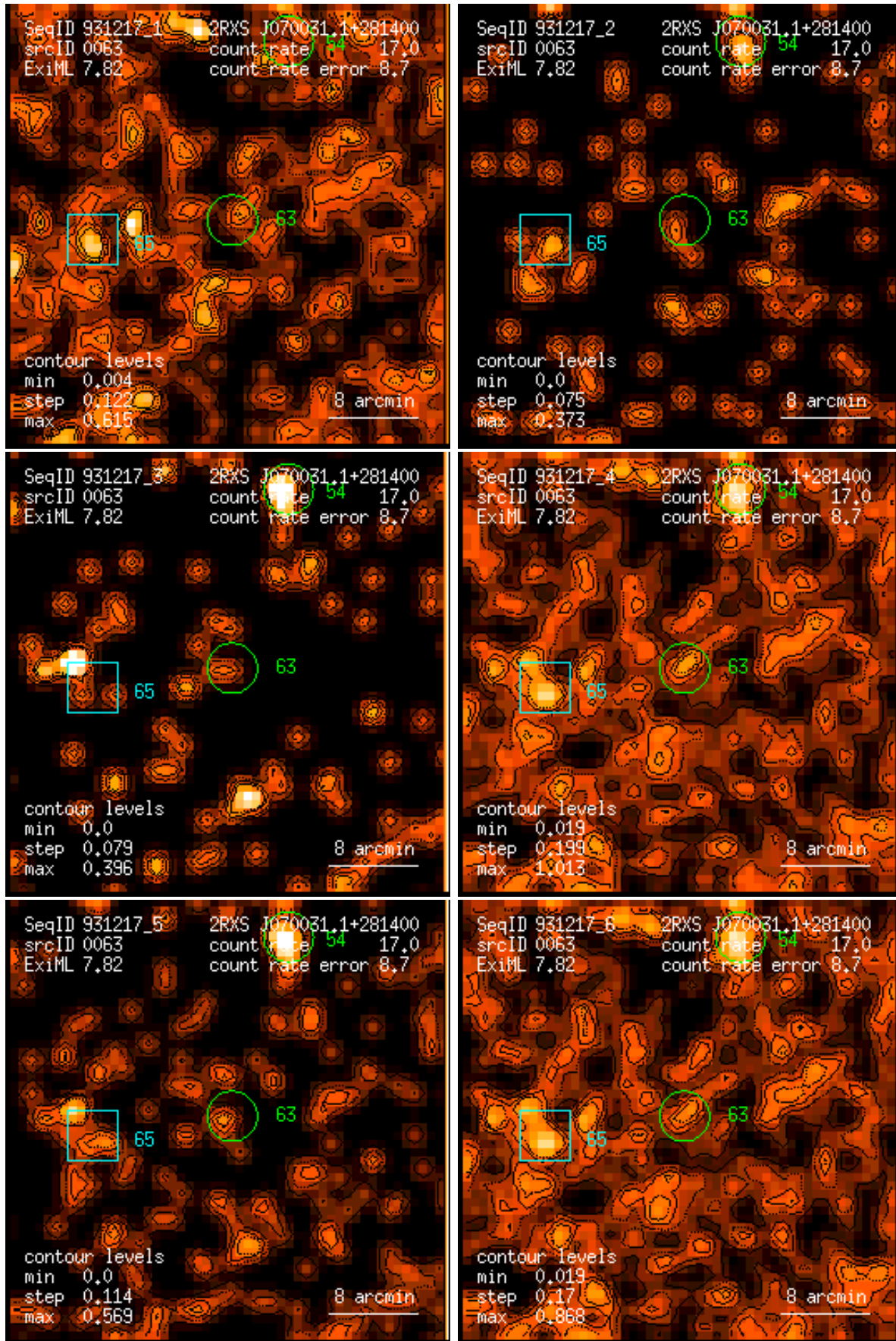
Figure 63: RASS 931217: detection 0063: band rate images, Gaussian filter: (1) PSPC channels 11 – 41, (2) 52 – 90, (3) 91 – 201, (4) 11 – 235, (5) 52 – 201, (6) 11 – 201. Broad band rates in counts/ks. Band rate contour levels in counts/ks/arcmin 2 .
