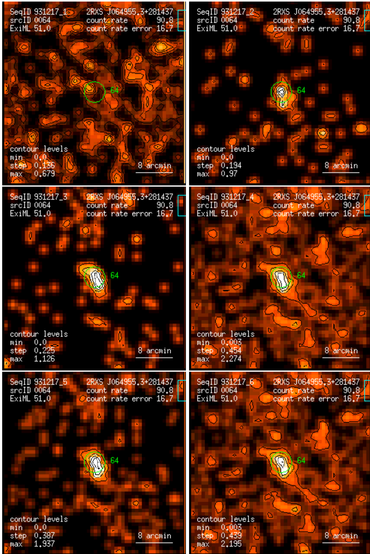
Figure 64: RASS 931217: detection 0064: band rate images, Gaussian filter: (1) PSPC channels 11 – 41, (2) 52 – 90, (3) 91 – 201, (4) 11 – 235, (5) 52 – 201, (6) 11 – 201. Broad band rates in counts/ks. Band rate contour levels in counts/ks/arcmin 2 .
