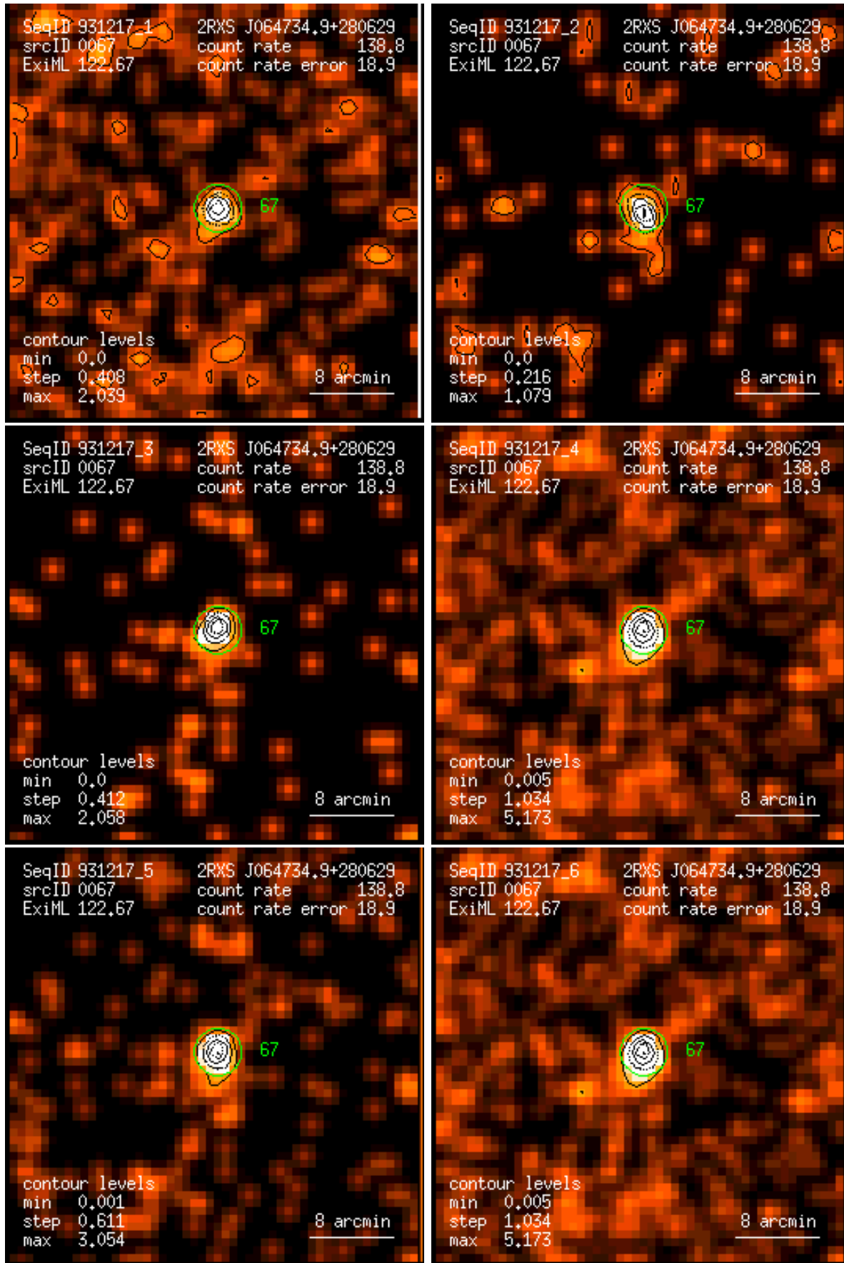
Figure 67: RASS 931217: detection 0067: band rate images, Gaussian filter: (1) PSPC channels 11 – 41, (2) 52 – 90, (3) 91 – 201, (4) 11 – 235, (5) 52 – 201, (6) 11 – 201. Broad band rates in counts/ks. Band rate contour levels in counts/ks/arcmin 2 .
