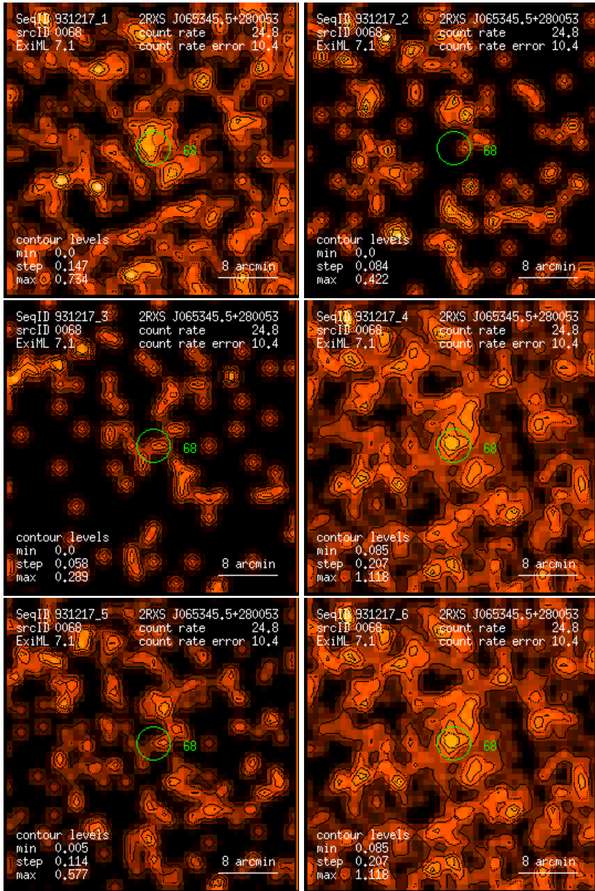
Figure 68: RASS 931217: detection 0068: band rate images, Gaussian filter: (1) PSPC channels 11 – 41, (2) 52 – 90, (3) 91 – 201, (4) 11 – 235, (5) 52 – 201, (6) 11 – 201. Broad band rates in counts/ks. Band rate contour levels in counts/ks/arcmin 2 .
