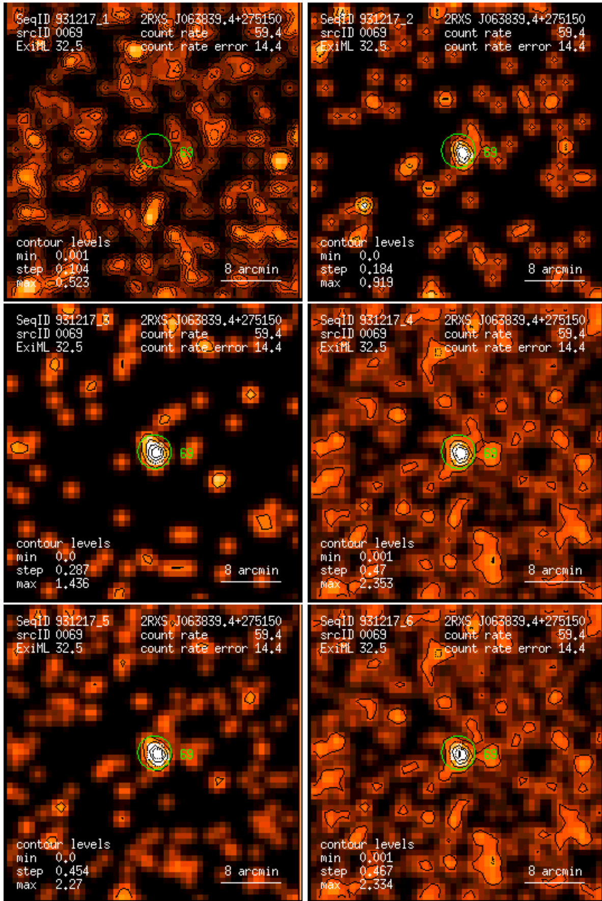
Figure 69: RASS 931217: detection 0069: band rate images, Gaussian filter: (1) PSPC channels 11 – 41, (2) 52 – 90, (3) 91 – 201, (4) 11 – 235, (5) 52 – 201, (6) 11 – 201. Broad band rates in counts/ks. Band rate contour levels in counts/ks/arcmin 2 .
