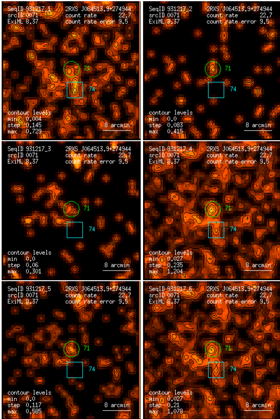
Figure 71: RASS 931217: detection 0071: band rate images, Gaussian filter: (1) PSPC channels 11 – 41, (2) 52 – 90, (3) 91 – 201, (4) 11 – 235, (5) 52 – 201, (6) 11 – 201. Broad band rates in counts/ks. Band rate contour levels in counts/ks/arcmin 2 .
