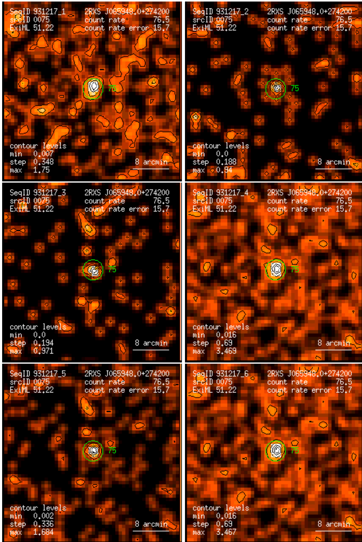
Figure 75: RASS 931217: detection 0075: band rate images, Gaussian filter: (1) PSPC channels 11 – 41, (2) 52 – 90, (3) 91 – 201, (4) 11 – 235, (5) 52 – 201, (6) 11 – 201. Broad band rates in counts/ks. Band rate contour levels in counts/ks/arcmin 2 .
