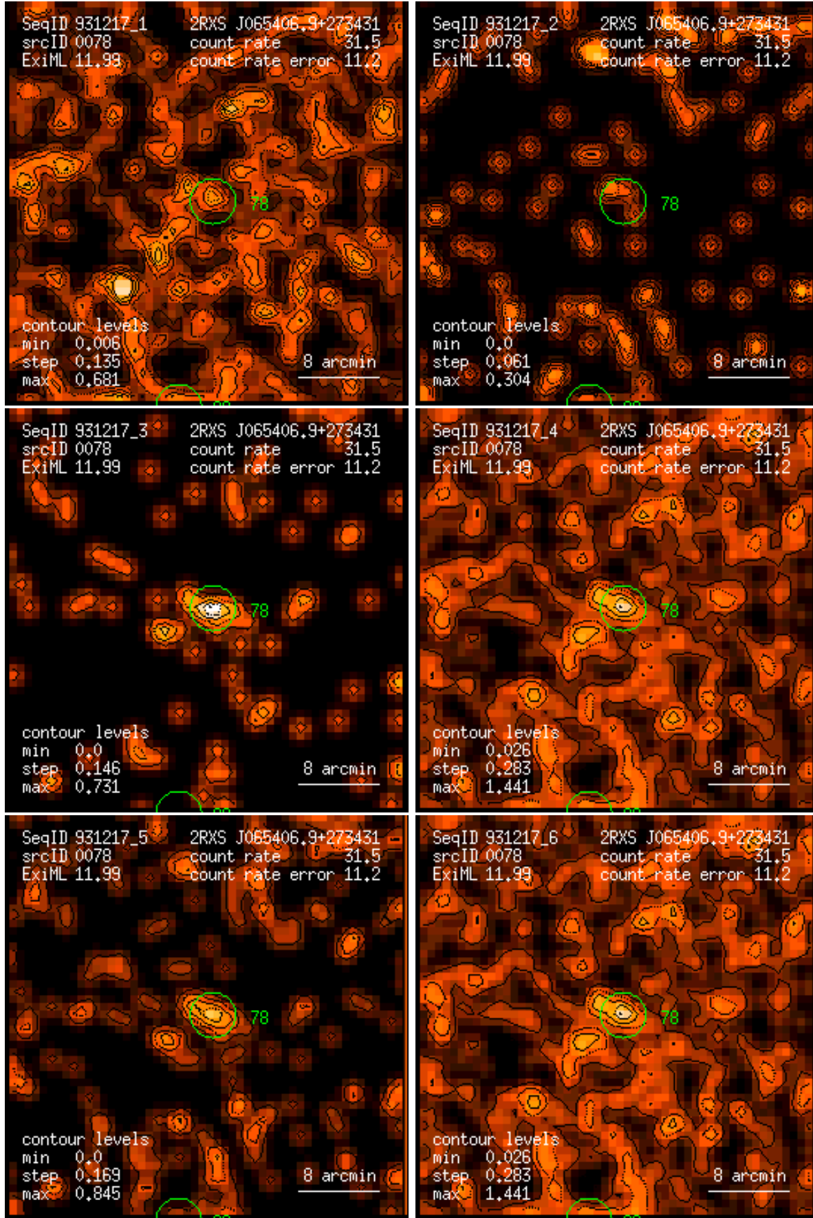
Figure 78: RASS 931217: detection 0078: band rate images, Gaussian filter: (1) PSPC channels 11 – 41, (2) 52 – 90, (3) 91 – 201, (4) 11 – 235, (5) 52 – 201, (6) 11 – 201. Broad band rates in counts/ks. Band rate contour levels in counts/ks/arcmin 2 .
