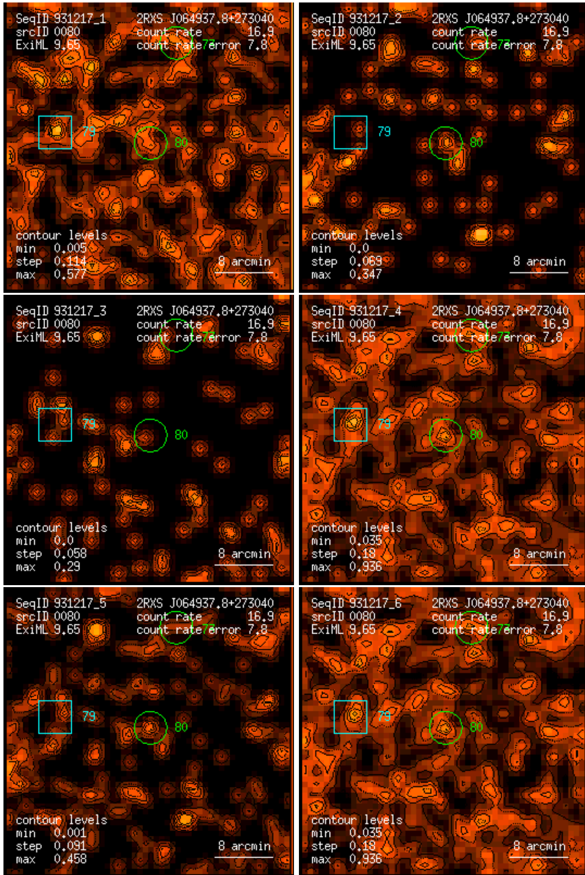
Figure 80: RASS 931217: detection 0080: band rate images, Gaussian filter: (1) PSPC channels 11 – 41, (2) 52 – 90, (3) 91 – 201, (4) 11 – 235, (5) 52 – 201, (6) 11 – 201. Broad band rates in counts/ks. Band rate contour levels in counts/ks/arcmin 2 .
