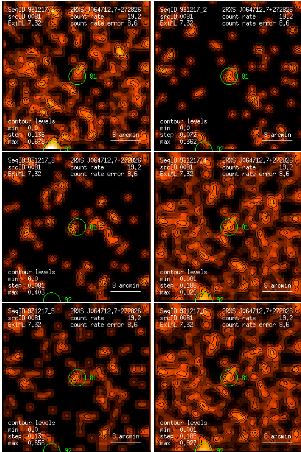
Figure 81: RASS 931217: detection 0081: band rate images, Gaussian filter: (1) PSPC channels 11 – 41, (2) 52 – 90, (3) 91 – 201, (4) 11 – 235, (5) 52 – 201, (6) 11 – 201. Broad band rates in counts/ks. Band rate contour levels in counts/ks/arcmin 2 .
