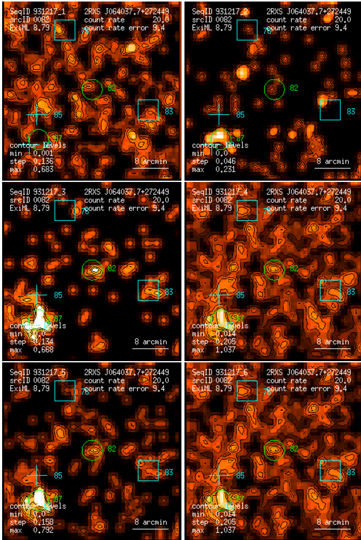
Figure 82: RASS 931217: detection 0082: band rate images, Gaussian filter: (1) PSPC channels 11 – 41, (2) 52 – 90, (3) 91 – 201, (4) 11 – 235, (5) 52 – 201, (6) 11 – 201. Broad band rates in counts/ks. Band rate contour levels in counts/ks/arcmin 2 .
