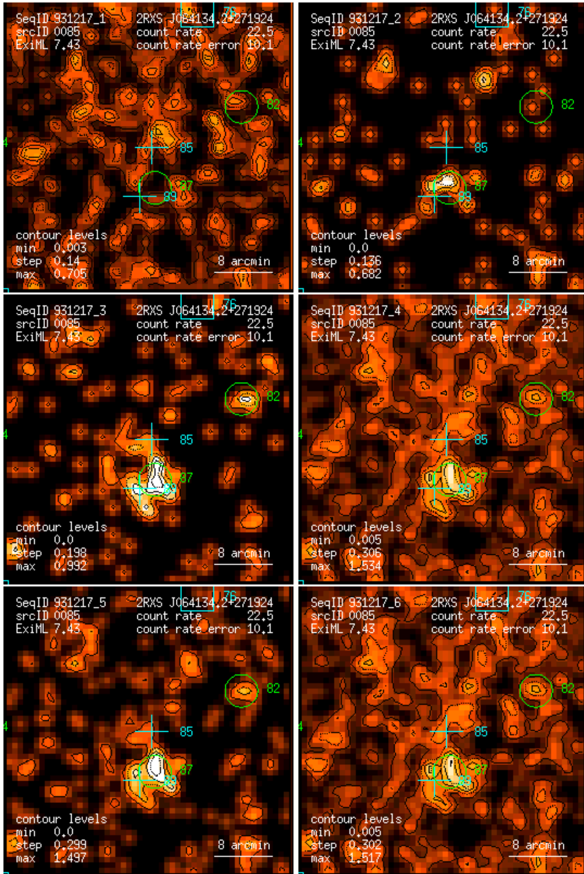
Figure 85: RASS 931217: detection 0085: band rate images, Gaussian filter: (1) PSPC channels 11 – 41, (2) 52 – 90, (3) 91 – 201, (4) 11 – 235, (5) 52 – 201, (6) 11 – 201. Broad band rates in counts/ks. Band rate contour levels in counts/ks/arcmin 2 .
