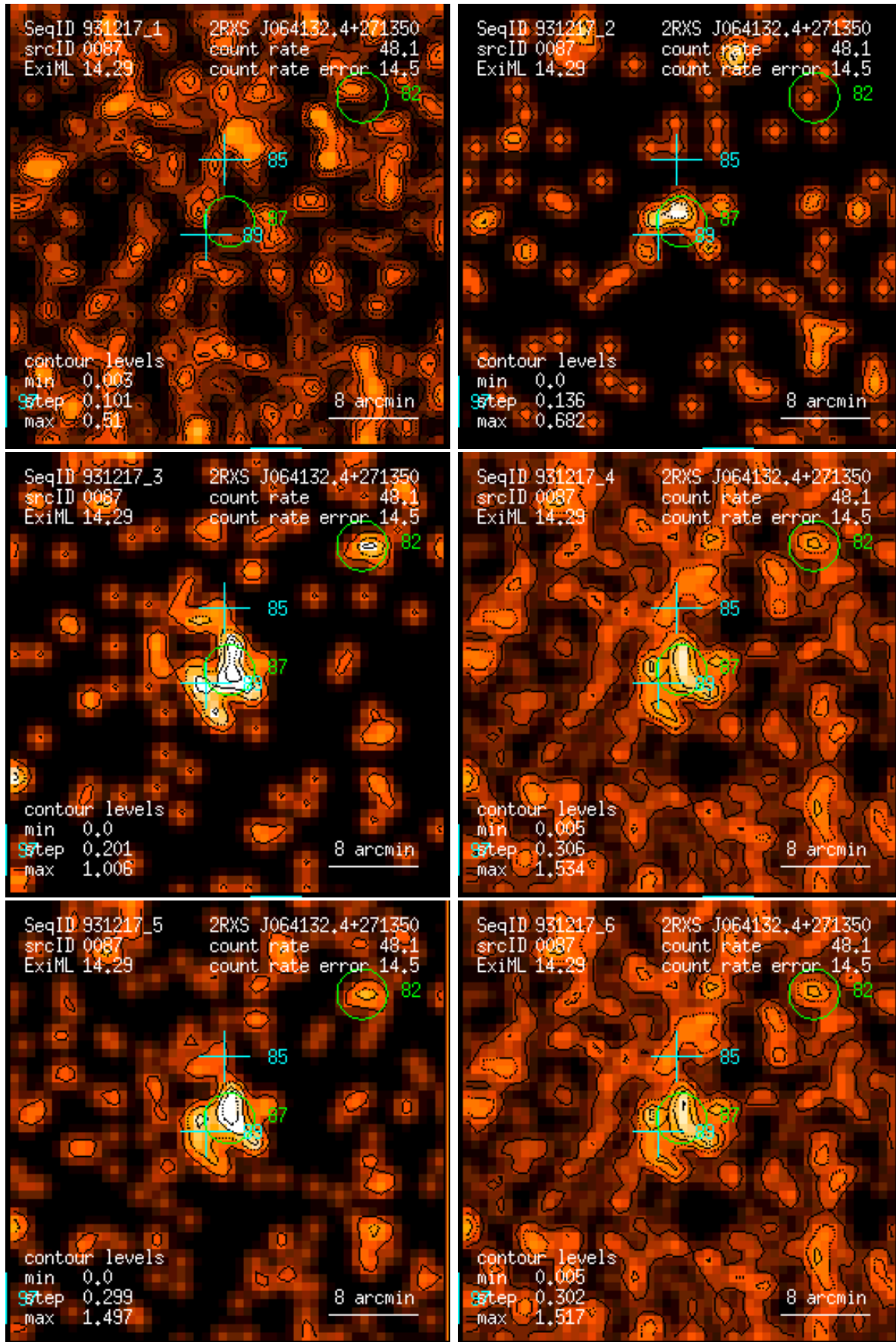
Figure 87: RASS 931217: detection 0087: band rate images, Gaussian filter: (1) PSPC channels 11 – 41, (2) 52 – 90, (3) 91 – 201, (4) 11 – 235, (5) 52 – 201, (6) 11 – 201. Broad band rates in counts/ks. Band rate contour levels in counts/ks/arcmin 2 .
