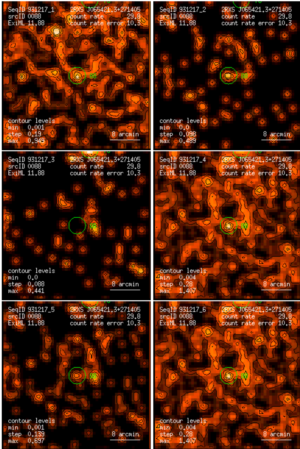
Figure 88: RASS 931217: detection 0088: band rate images, Gaussian filter: (1) PSPC channels 11 – 41, (2) 52 – 90, (3) 91 – 201, (4) 11 – 235, (5) 52 – 201, (6) 11 – 201. Broad band rates in counts/ks. Band rate contour levels in counts/ks/arcmin 2 .
