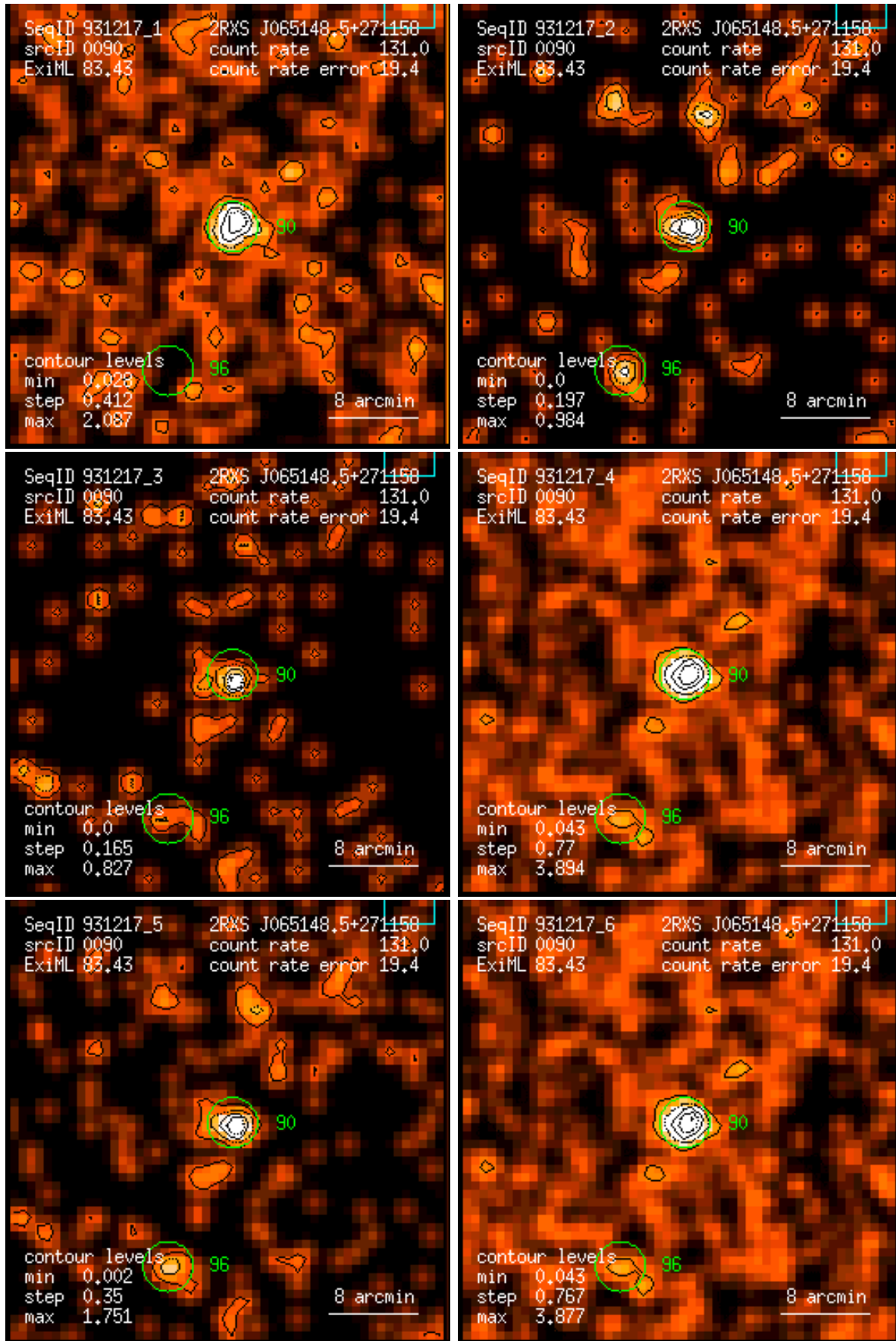
Figure 90: RASS 931217: detection 0090: band rate images, Gaussian filter: (1) PSPC channels 11 – 41, (2) 52 – 90, (3) 91 – 201, (4) 11 – 235, (5) 52 – 201, (6) 11 – 201. Broad band rates in counts/ks. Band rate contour levels in counts/ks/arcmin 2 .
