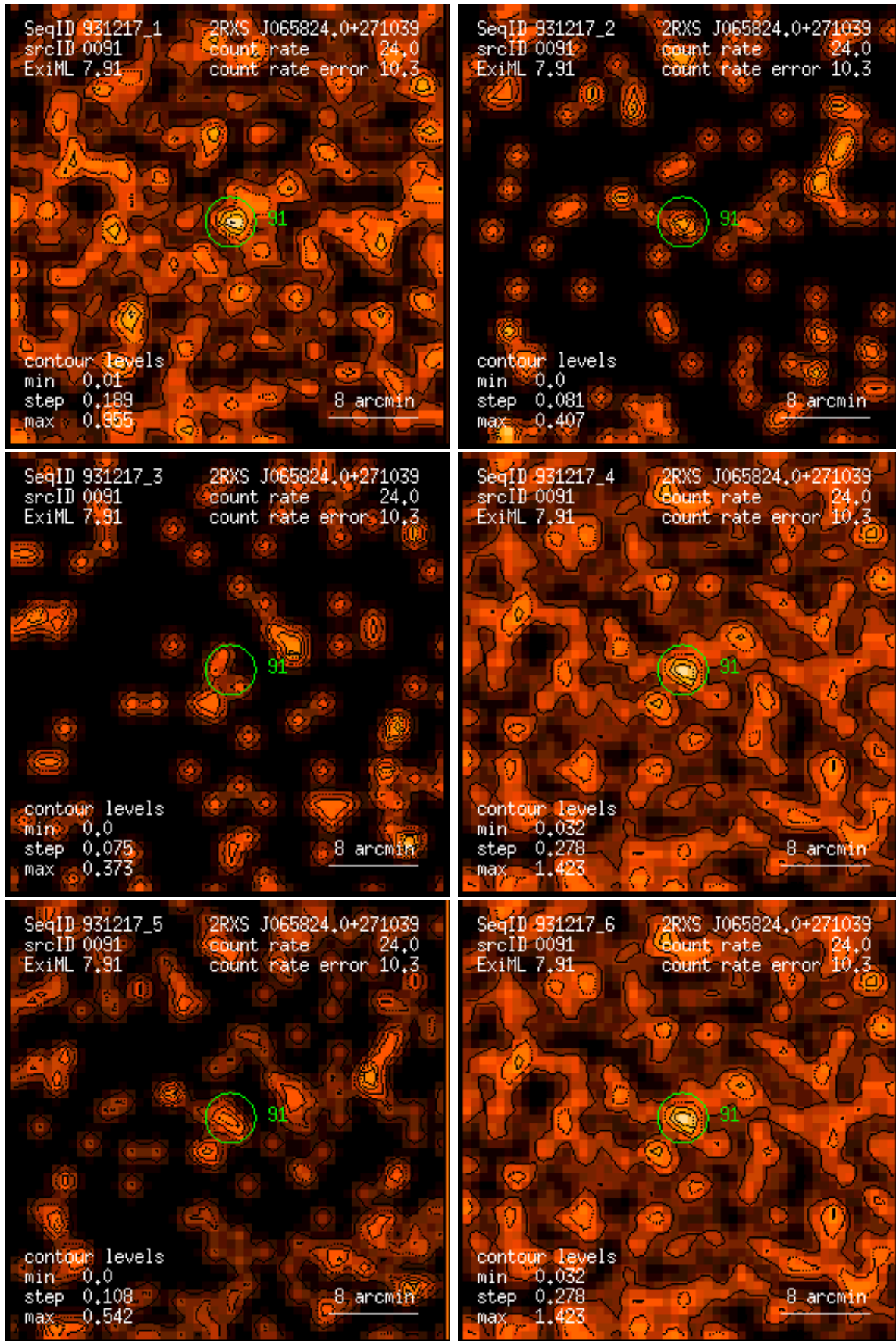
Figure 91: RASS 931217: detection 0091: band rate images, Gaussian filter: (1) PSPC channels 11 – 41, (2) 52 – 90, (3) 91 – 201, (4) 11 – 235, (5) 52 – 201, (6) 11 – 201. Broad band rates in counts/ks. Band rate contour levels in counts/ks/arcmin 2 .
