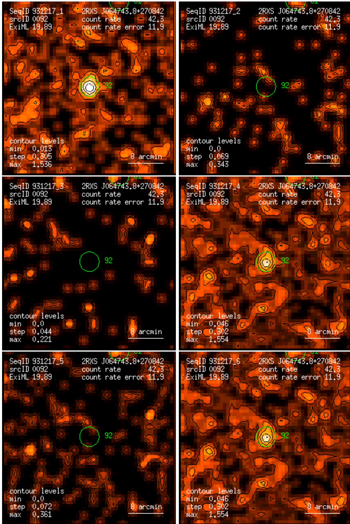
Figure 92: RASS 931217: detection 0092: band rate images, Gaussian filter: (1) PSPC channels 11 – 41, (2) 52 – 90, (3) 91 – 201, (4) 11 – 235, (5) 52 – 201, (6) 11 – 201. Broad band rates in counts/ks. Band rate contour levels in counts/ks/arcmin 2 .
