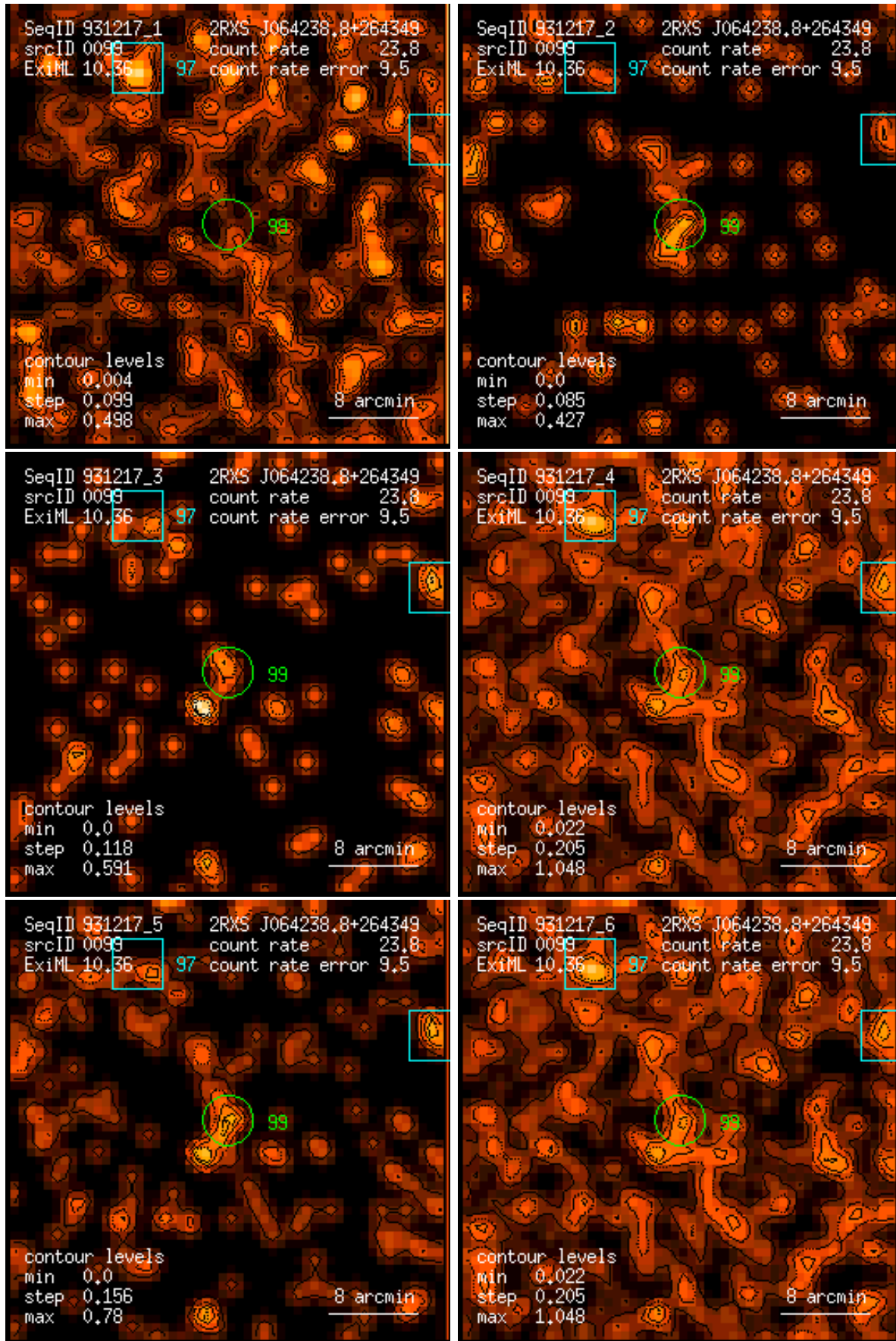
Figure 99: RASS 931217: detection 0099: band rate images, Gaussian filter: (1) PSPC channels 11 – 41, (2) 52 – 90, (3) 91 – 201, (4) 11 – 235, (5) 52 – 201, (6) 11 – 201. Broad band rates in counts/ks. Band rate contour levels in counts/ks/arcmin 2 .
